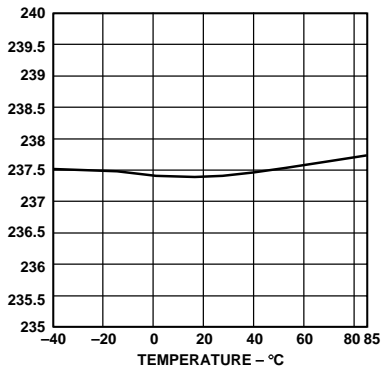
Figure 6. Power-Down RESET Delay vs. Temperature ADM8_R
