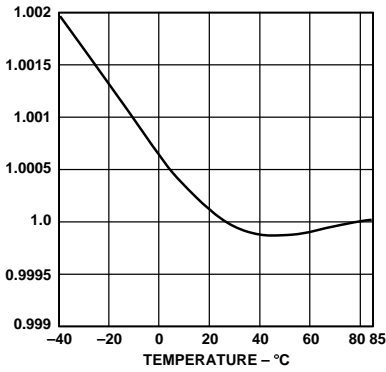
Figure 7. Normalized RESET Voltage Threshold vs. Temperature
