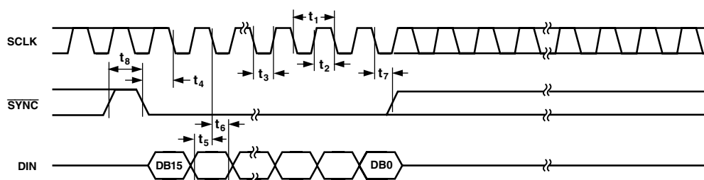
Figure 1. Serial Write Operation
