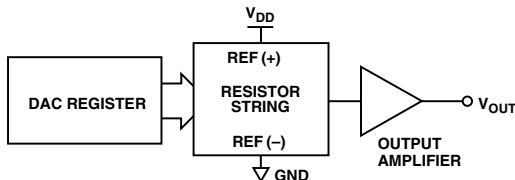
Figure 20. DAC Architecture
