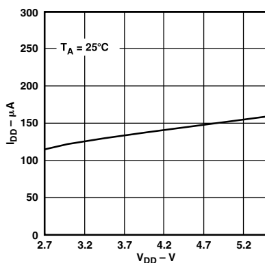
Figure 12. Supply Current vs. Supply Voltage
