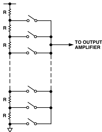
Figure 21. Resistor String
