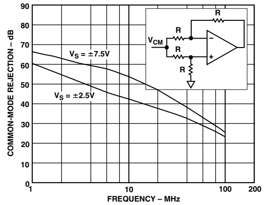
Figure 15. Common-Mode Rejection vs. Frequency
