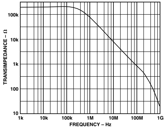
Figure 18. Open-Loop Transimpedance vs. Frequency
