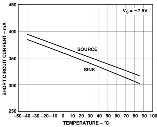
Figure 13. Short Circuit Current vs. Temperature
