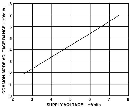
Figure 4. Input Common-Mode Voltage Range vs. Supply Voltage
