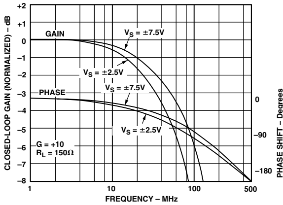
Figure 24. Closed-Loop Gain and Phase vs. Frequency, G = +10 , R_L = 150\ \Omega
