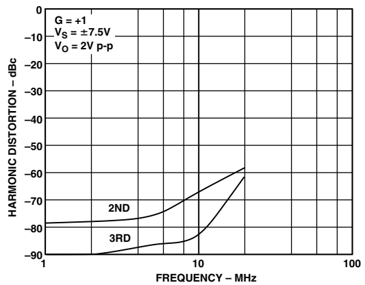
Figure 17. Harmonic Distortion vs. Frequency, R_L = 150\ \Omega
