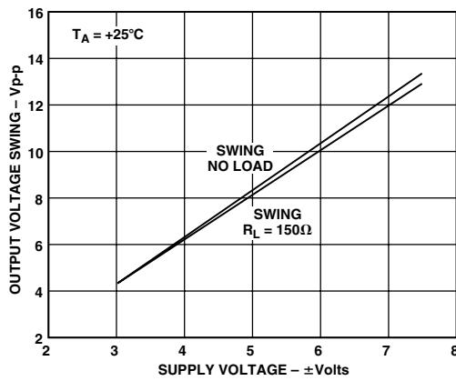
Figure 7. Output Voltage Swing vs. Supply Voltage
