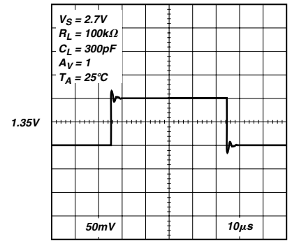
Figure 12. Small Signal Transient Response
