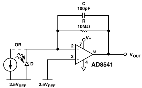
Figure 35. High Input Impedance Application—Photodiode Amplifier
