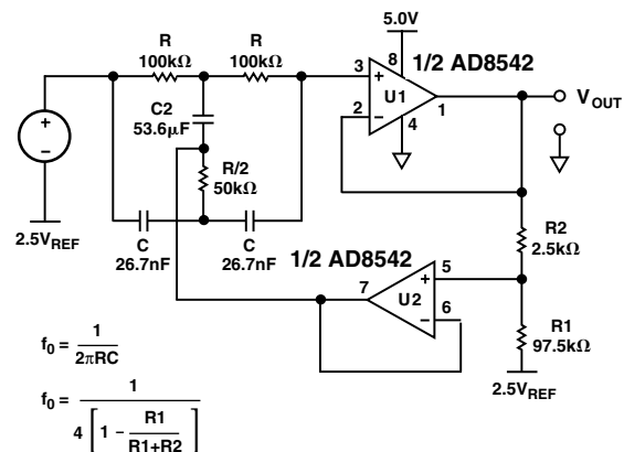
Figure 31. 60 Hz Twin-T Notch Filter, Q = 10
