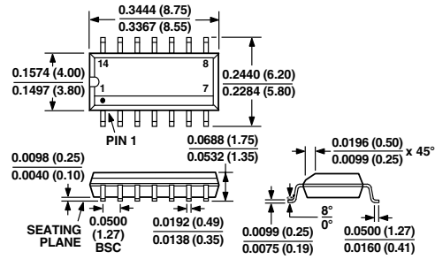
14-Lead SOIC (SO-14)
