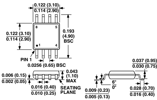
8-Lead MSOP (RM-8)
