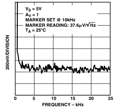
Figure 30. Voltage Noise
