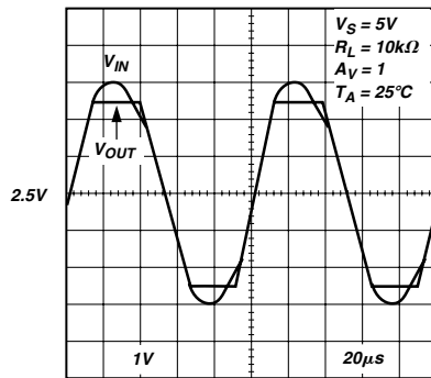
Figure 26. No Phase Reversal vs. Frequency
