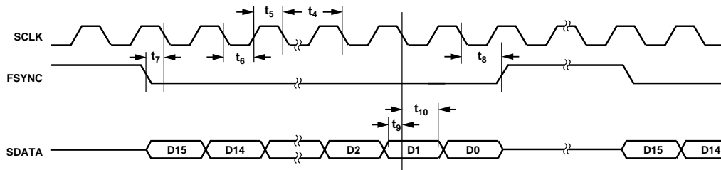
Figure 3. Serial Timing
