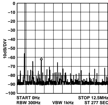
Figure 12. f_{MCLK} = 25 \text{ MHz} , f_{OUT} = 1.1 \text{ MHz} , Frequency Word = B439581
