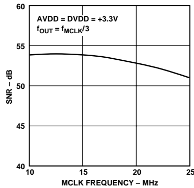
Figure 9. SNR vs. MCLK Frequency
