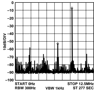
Figure 20. f_{MCLK} = 25 \text{ MHz} , f_{OUT} = 9.1 \text{ MHz} , Frequency Word = 5D2F1AA0
