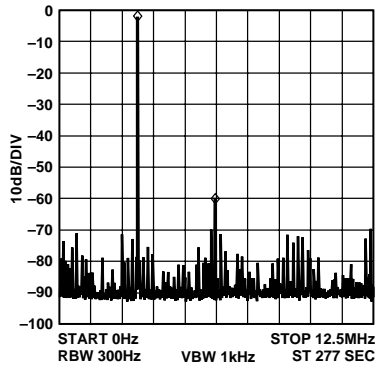
Figure 14. f_{MCLK} = 25 \text{ MHz} , f_{OUT} = 3.1 \text{ MHz} , Frequency Word = 1FBE76C9
