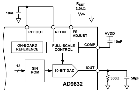
Figure 1. Test Circuit with Which Specifications Are Tested
