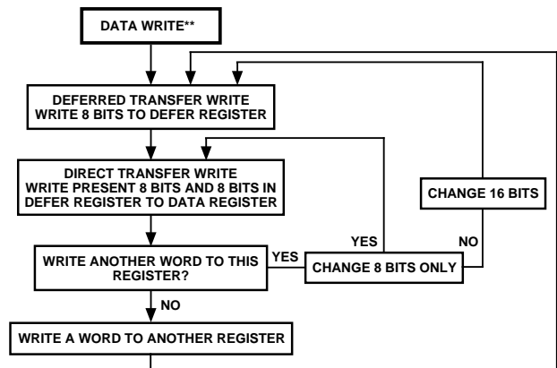
Figure 24. Data Writes
