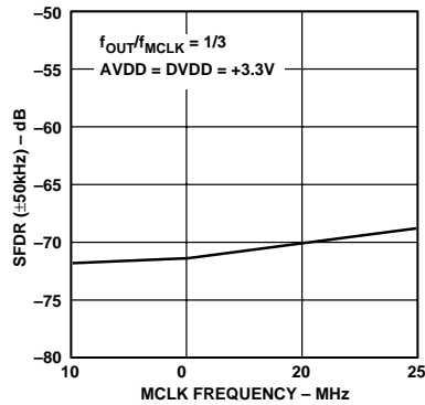
Figure 6. Narrow Band SFDR vs. MCLK Frequency
