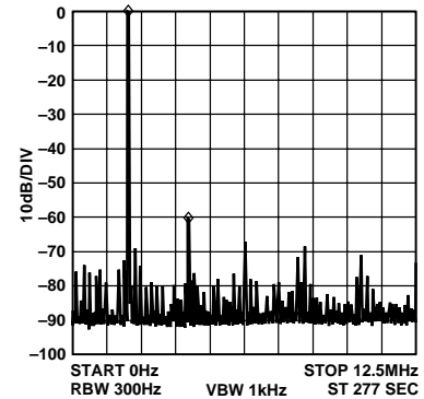
Figure 13. f_{MCLK} = 25 \text{ MHz} , f_{OUT} = 2.1 \text{ MHz} , Frequency Word = 15810625
