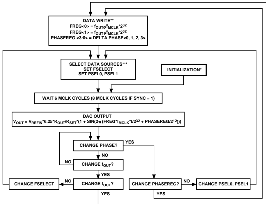
Figure 22. Flow Chart for AD9832 Initialization and Operation
