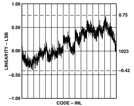
Figure 16. Typical Linearity
