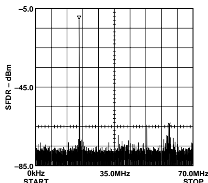
Figure 18. Single-Tone SFDR @ f_{CLOCK} = 140\text{ MHz} ( f_{OUT1} = 20\text{ MHz} )
