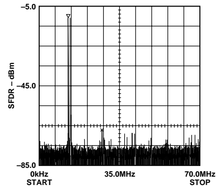
Figure 19. Dual-Tone SFDR @ f_{CLOCK} = 140\text{ MHz} ( f_{OUT1} = 13.5\text{ MHz} , f_{OUT2} = 14.5\text{ MHz} )
