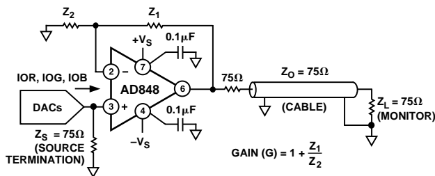
Figure 24. AD848 As an Output Buffer
