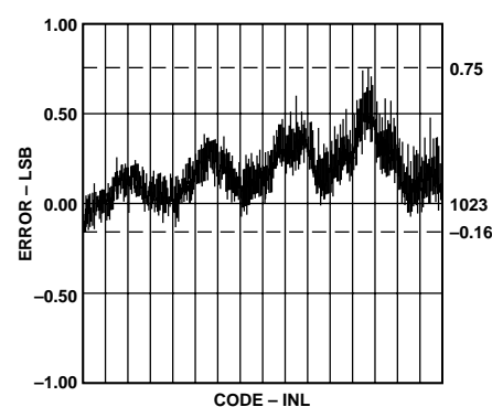
Figure 7. Typical Linearity (INL)
