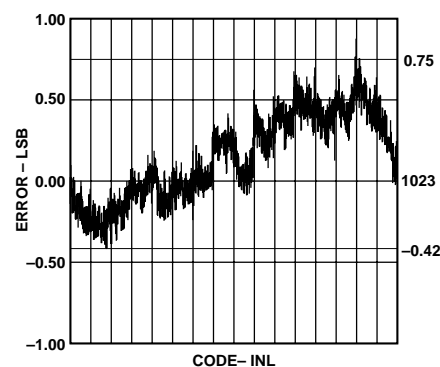
Figure 16. Typical Linearity
