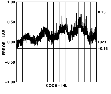
Figure 7. Typical Linearity
