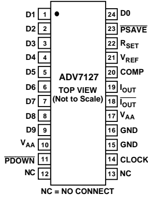
24-Lead TSSOP
