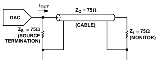
Figure 22. Analog Output Termination for RS-343A
