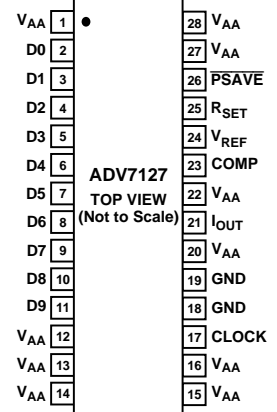
28-Lead SOIC
