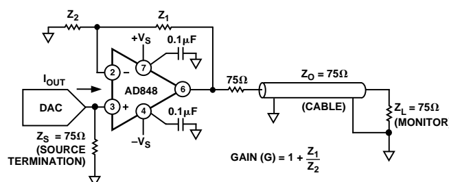
Figure 24. AD848 As an Output Buffer
