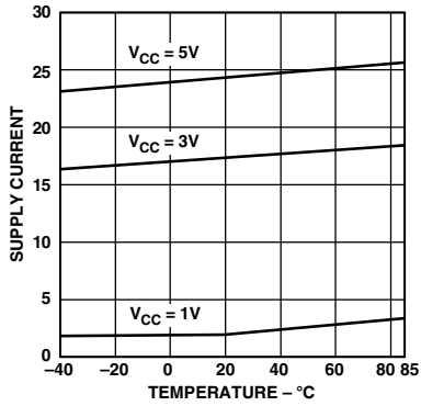
TPC 1. Supply Current vs. Temperature (No Load)
