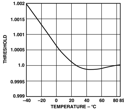
TPC 5. Normalized RESET Voltage Threshold vs. Temperature
