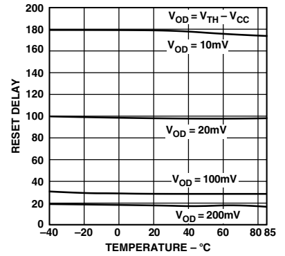
TPC 3. Power-Down RESET Delay vs. Temperature ADM809-5L
