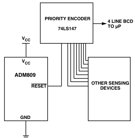
Figure 4. Interfacing to \mu\text{Ps} with Multiple Interrupts
