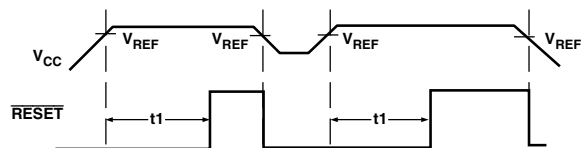
Figure 2. Power Fail \overline{\text{RESET}} Timing
