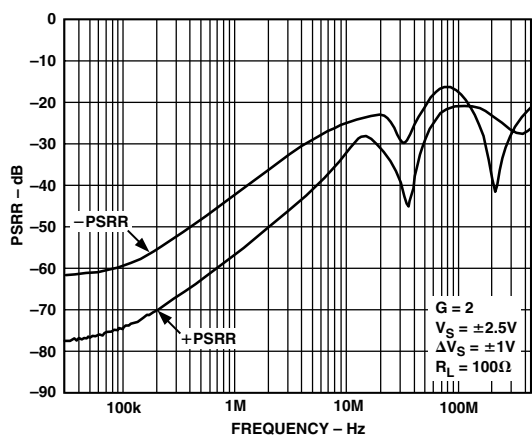
TPC 9. PSRR vs. Frequency
