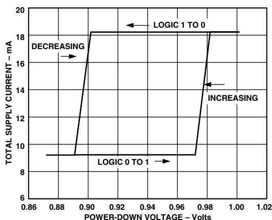
TPC 24. Power-Up/Down Threshold Voltage
