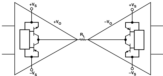
Figure 8. Simplified Differential Driver
