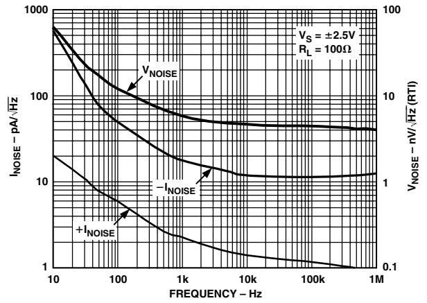
TPC 4. I_{NOISE} and V_{NOISE} vs. Frequency
