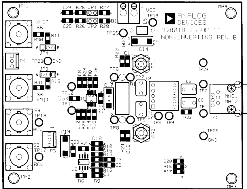
Figure 13. Assembly—Primary Side
