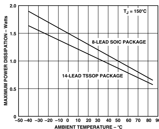
Figure 3. Plot of Maximum Power Dissipation vs. Temperature
