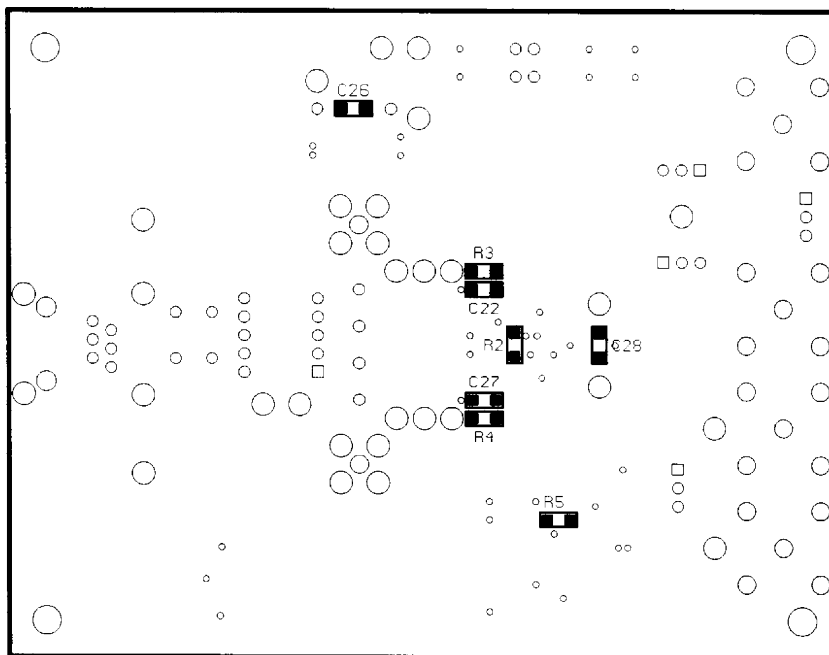
Figure 19. Assembly—Secondary Side
