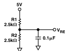
Figure 7. Midsupply Reference
