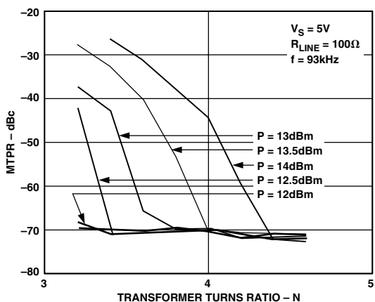
TPC 20. MTPR vs. Turns Ratio
