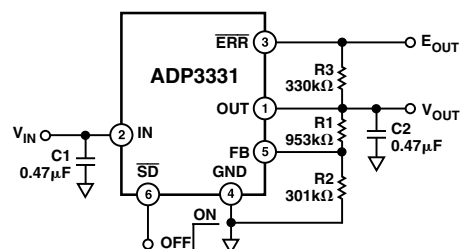
Figure 6. ADP3331 LDO
