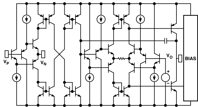
Figure 4. Simplified Schematic
