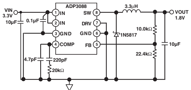
Figure 1. Typical Application
