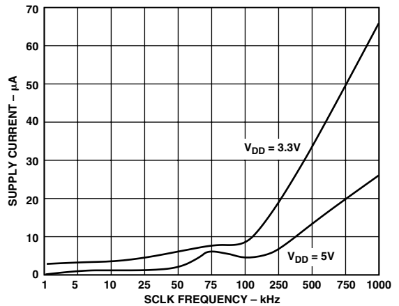
Figure 7. Standby Supply Current vs. Clock Frequency
