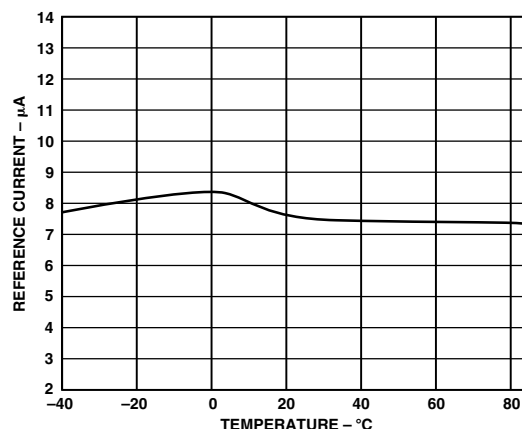
TPC 10. Reference Current vs. Temperature
