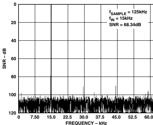
TPC 12. Auxiliary Channel Dynamic Performance
