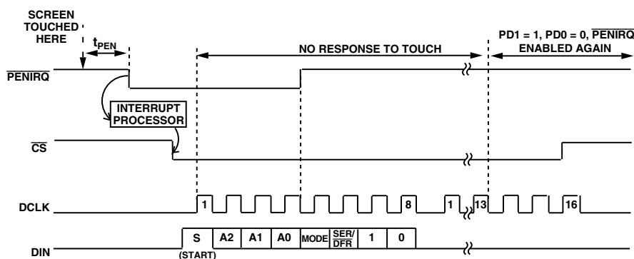
Figure 14. \overline{\text{PENIRQ}} Timing Diagram
