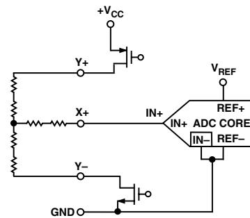
Figure 6. Single-Ended Reference Mode (SER/DFR = 1)
