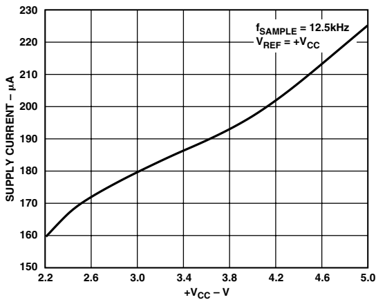
TPC 2. Supply Current vs. +V CC
