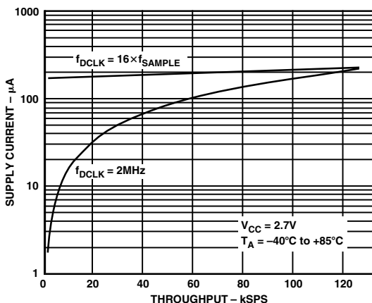
Figure 8. Supply Current vs. Throughput ( \mu\text{A} )
