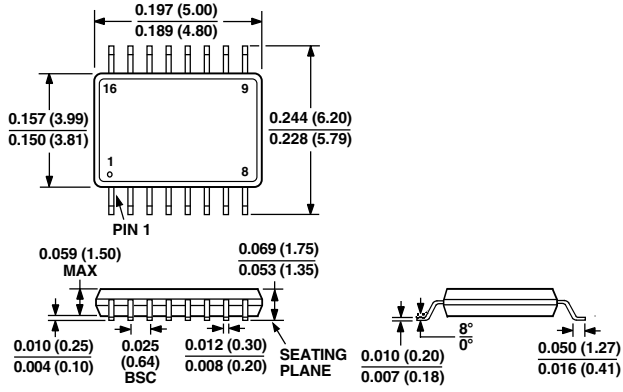
16-Lead QSOP (RQ-16)
