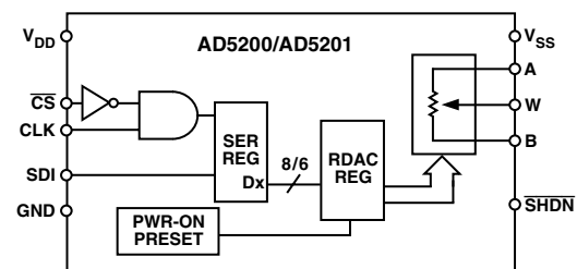
Figure 3. Block Diagram
