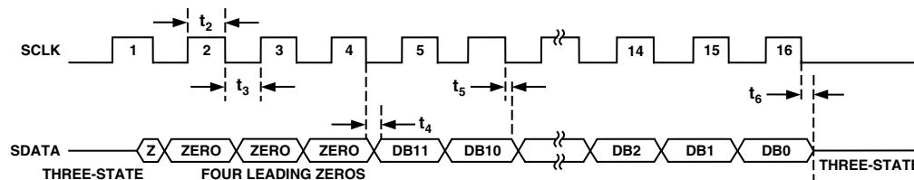
Figure 7. Data Read Operation in Mode 0
