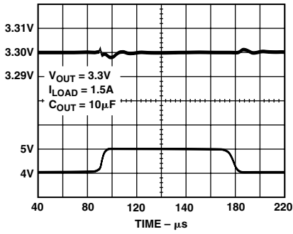
TPC 10. Line Transient Response
