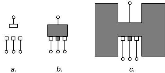
Figure 4. PCB Layouts
