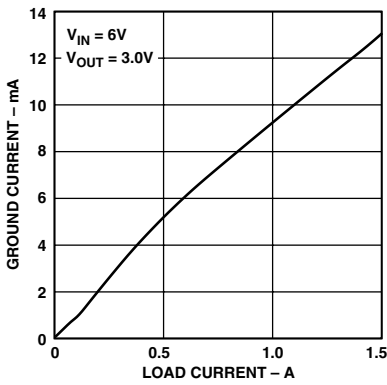
TPC 4. Ground Current vs. Load Current
