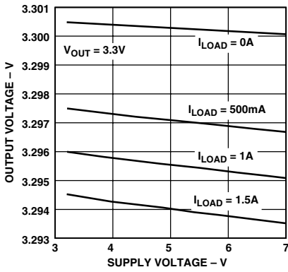
TPC 1. Output Voltage vs. Supply Voltage
