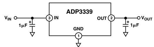
Figure 1. Typical Application Circuit
