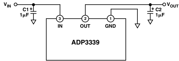
Figure 3. Typical Application Circuit
