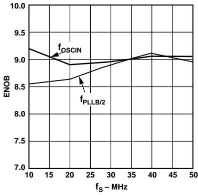
TPC 33. Rx Path ENOB vs. f_{ADC}
