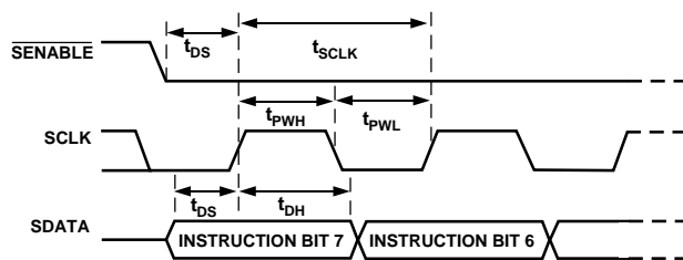
Figure 8. Timing Diagram Register Write to AD9875/AD9876
