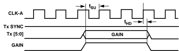
Figure 6. GAIN Programming
