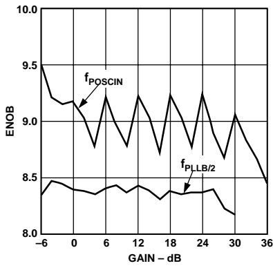
TPC 39. Rx Path ENOB vs. Gain
