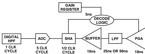
Figure 4. AGC Timing
