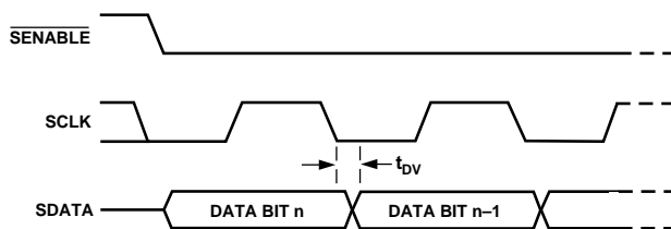
Figure 9. Timing Diagram Register Read from AD9875/AD9876
