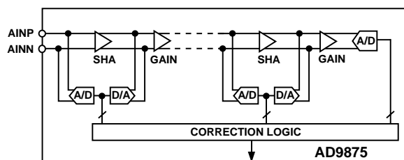
Figure 2. ADC Theory of Operation
