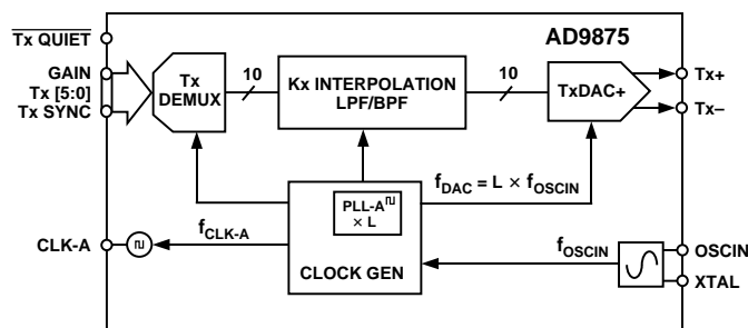
Figure 1. Transmit Path Block Diagram
