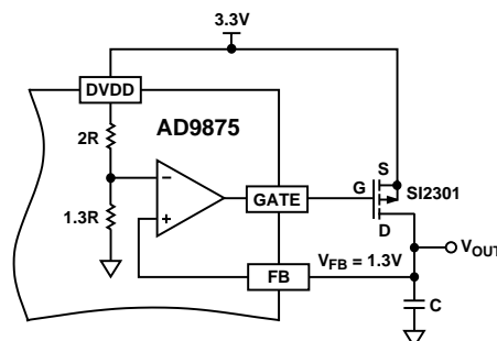
Figure 3b. Connections for a 1.3 V Linear Regulator
