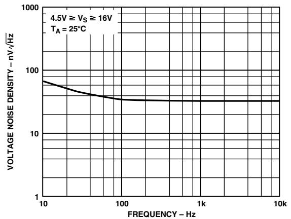
TPC 4. Voltage Noise Density vs. Frequency
