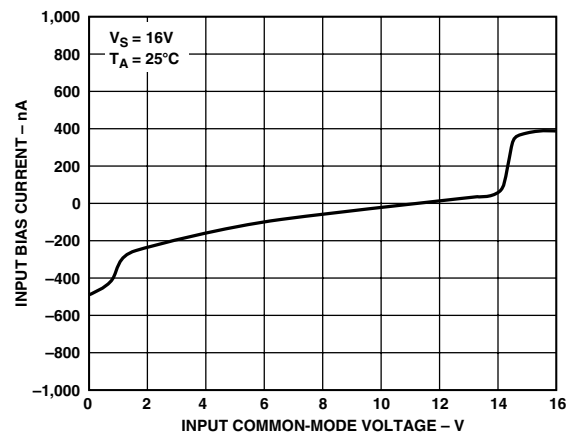
Figure 2. AD856x Input Bias Current vs. Common-Mode Voltage
