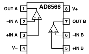
8-Lead MSOP (RM Suffix)
