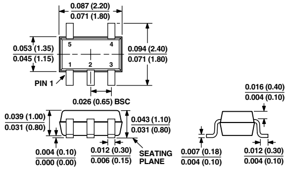
5-Lead Plastic Surface-Mount (KS-5)
