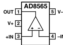
5-Lead SC70 (KS Suffix)
