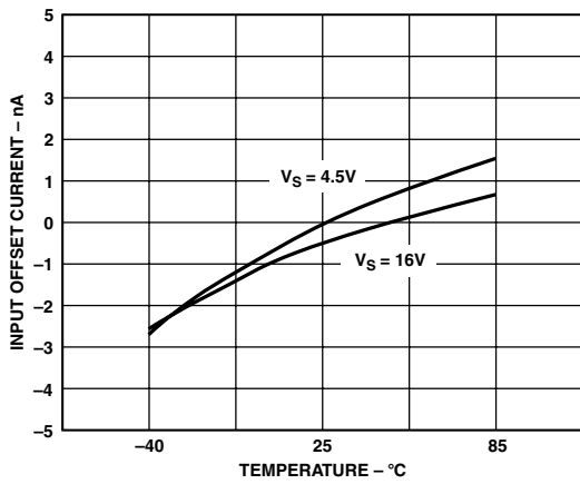
TPC 19. Input Offset Current vs. Temperature
