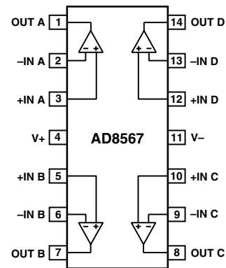
14-Lead TSSOP (RU Suffix)
