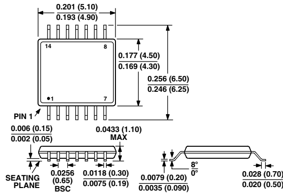
14-Lead Thin Shrink SO (RU-14)
