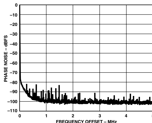
Figure 14. Phase Noise Performance
