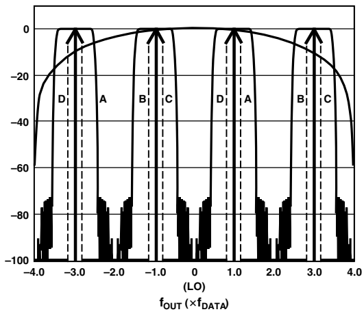
Figure 38. 4x Interpolation, Complex f_{DAC}/4 Modulation
