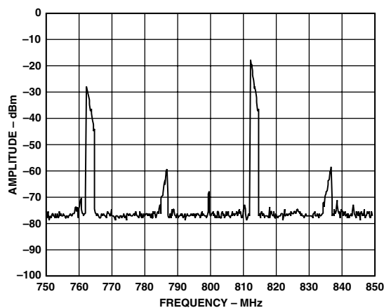
Figure 46. AD9775 Complex Output from Figure 45, Now Quadrature Modulated by AD8345 (LO = 800 MHz)
