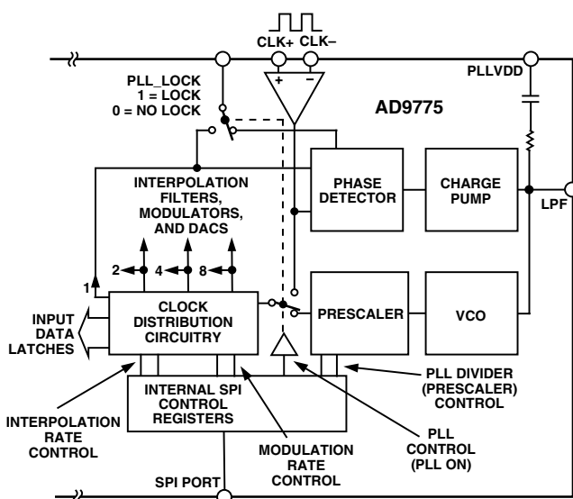
Figure 12. PLL and Clock Circuitry with PLL Enabled
