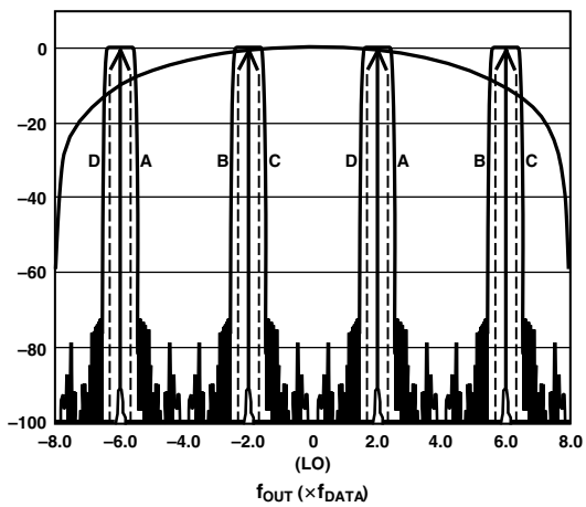
Figure 39. 8x Interpolation, Complex f_{DAC}/4 Modulation
