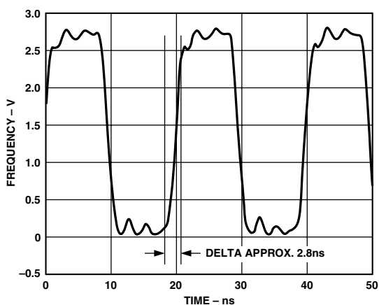
Figure 19. DATACLK Driver Capability into 330 Ω at 50 MHz
