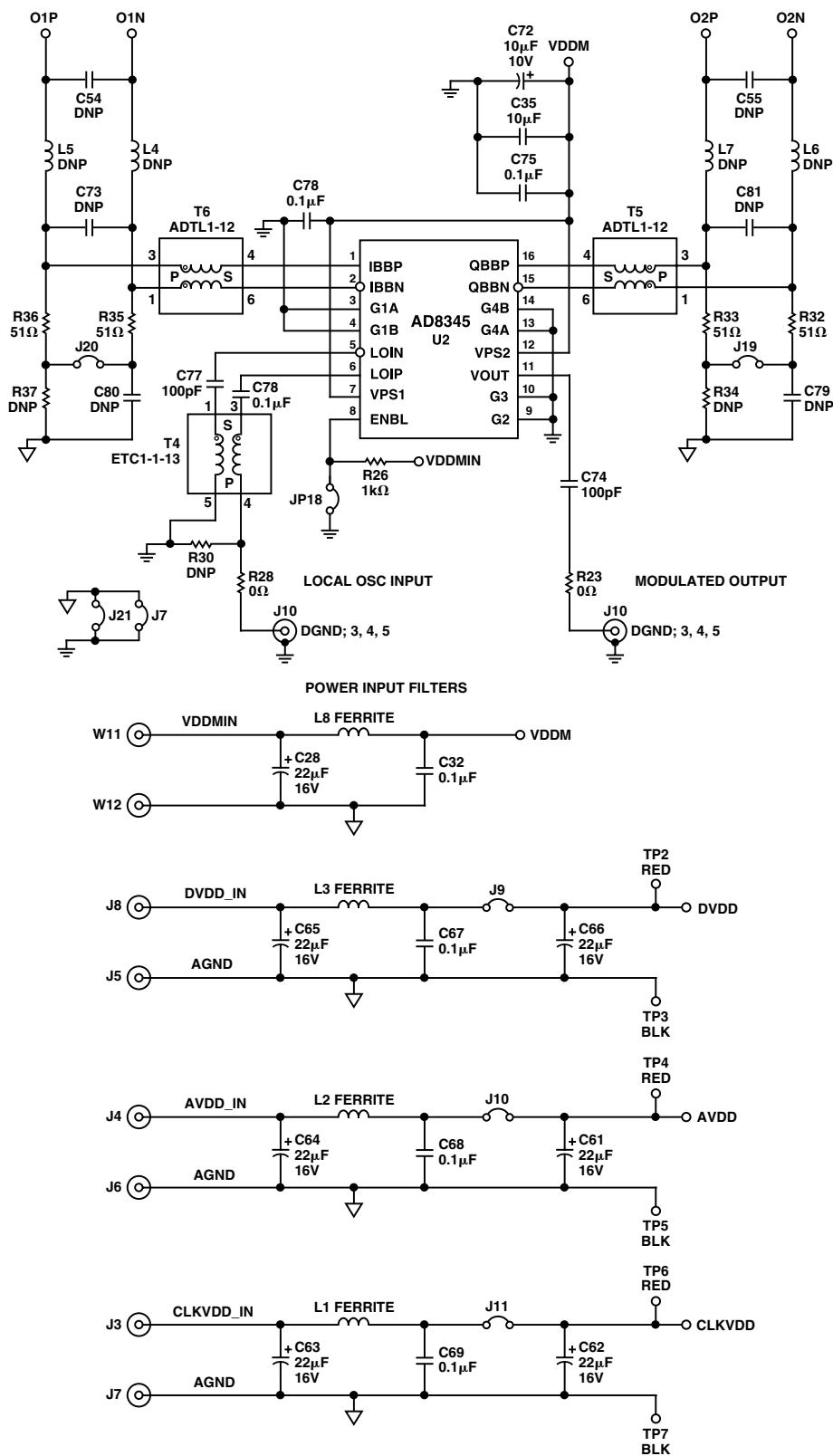
Figure 59. AD8345 Circuitry on AD9775 Evaluation Board
