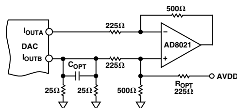
Figure 53. Op Amp-Coupled Output Circuit
