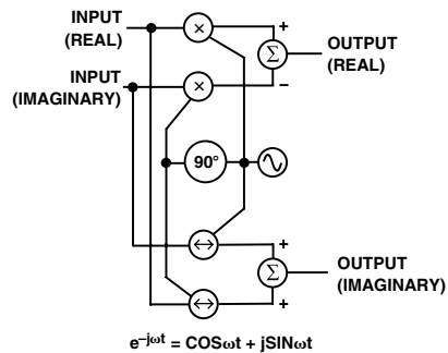
Figure 31. Implementation of a Complex Modulator
