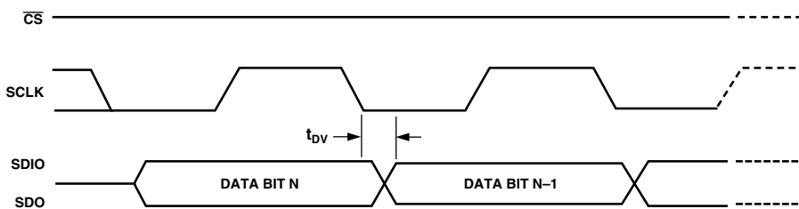
Figure 5. Timing Diagram for Register Read from AD9775
