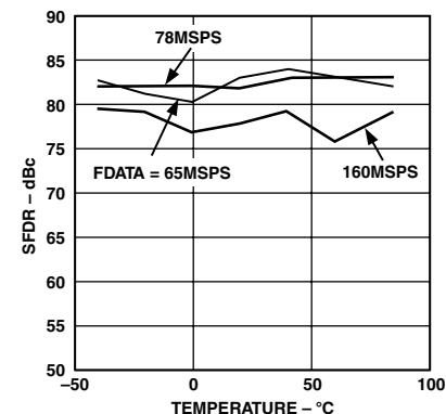
TPC 18. SFDR vs. Temperature @ f_{\text{OUT}} = f_{\text{DATA}}/11
