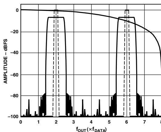
Figure 28c. 8× Interpolation, Modulation = f_{DAC}/4
