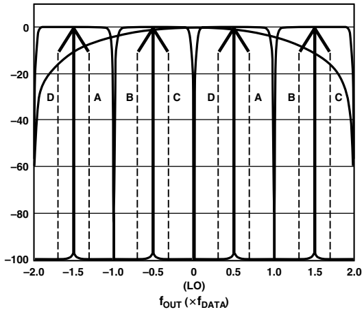
Figure 37. 2x Interpolation, Complex f_{DAC}/4 Modulation
