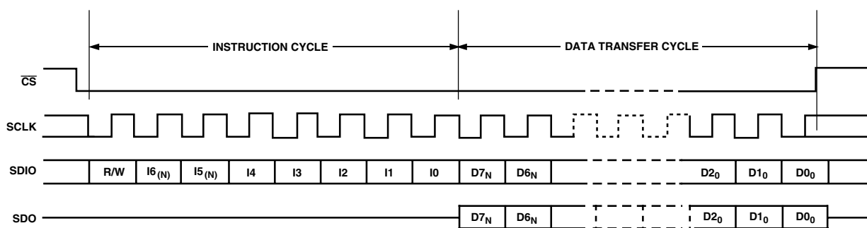
Figure 3a. Serial Register Interface Timing MSB First
