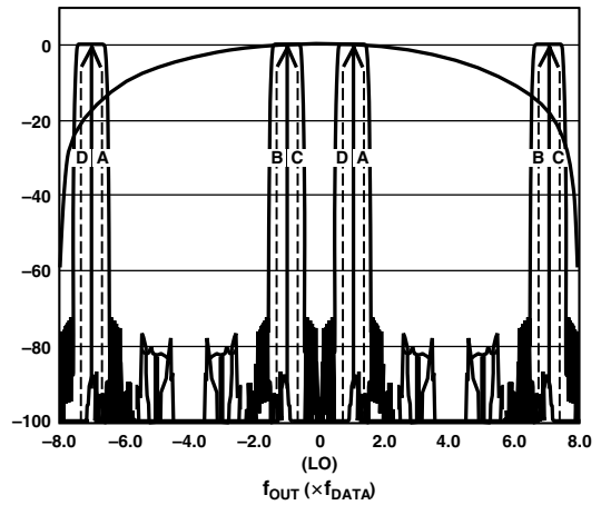
Figure 42. 8x Interpolation, Complex f_{DAC}/8 Modulation
