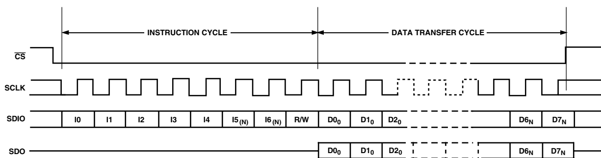
Figure 3b. Serial Register Interface Timing LSB First
