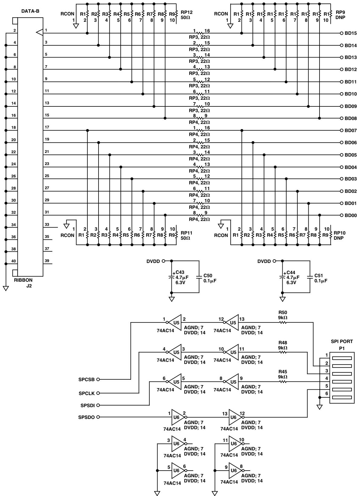
Figure 62. AD9775 Evaluation Board Input (B Channel) and SPI Port Circuitry
