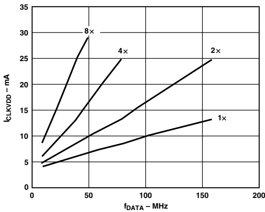
Figure 17. I_{CLKVDD} vs. f_{DATA} vs. Interpolation Rate, PLL Disabled
