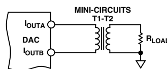
Figure 52. Transformer-Coupled Output Circuit
