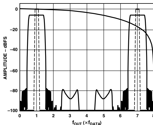
Figure 28d. 8× Interpolation, Modulation = f_{DAC}/8
