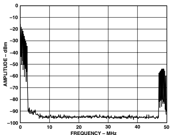
Figure 43. AD9775, Real DAC Output of Complex Input Signal Near Baseband (Positive Frequencies Only), Interpolation = 4x, No Modulation in AD9775
