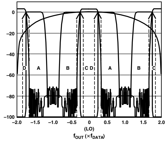
Figure 40. 2x Interpolation, Complex f_{DAC}/8 Modulation
