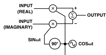
Figure 32. Quadrature Modulator
