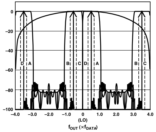
Figure 41. 4x Interpolation, Complex f_{DAC}/8 Modulation
