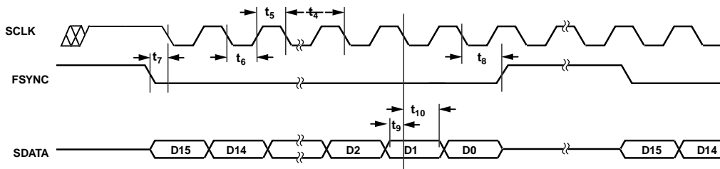
Figure 4. Serial Timing
