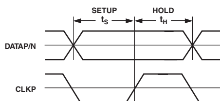
Figure 1. Setup and Hold Time
