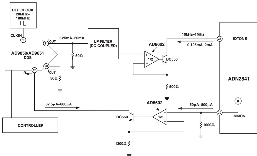
Figure 3. Circuitry to Allow Fiber Identification
