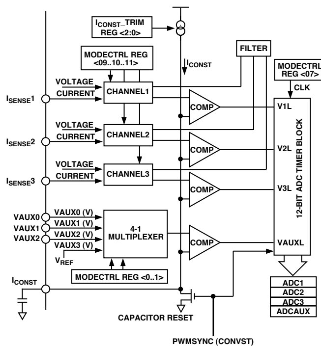
Figure 11. ADC Overview
