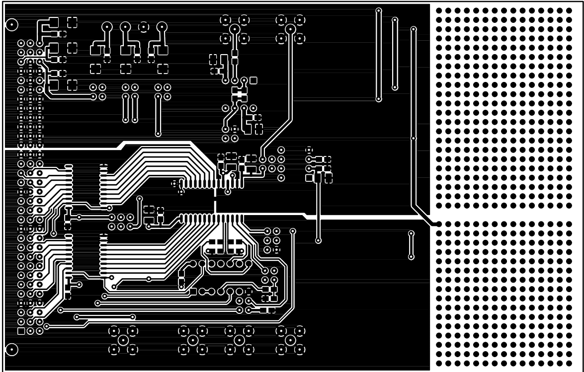
Figure 6. Component Side Artwork.
