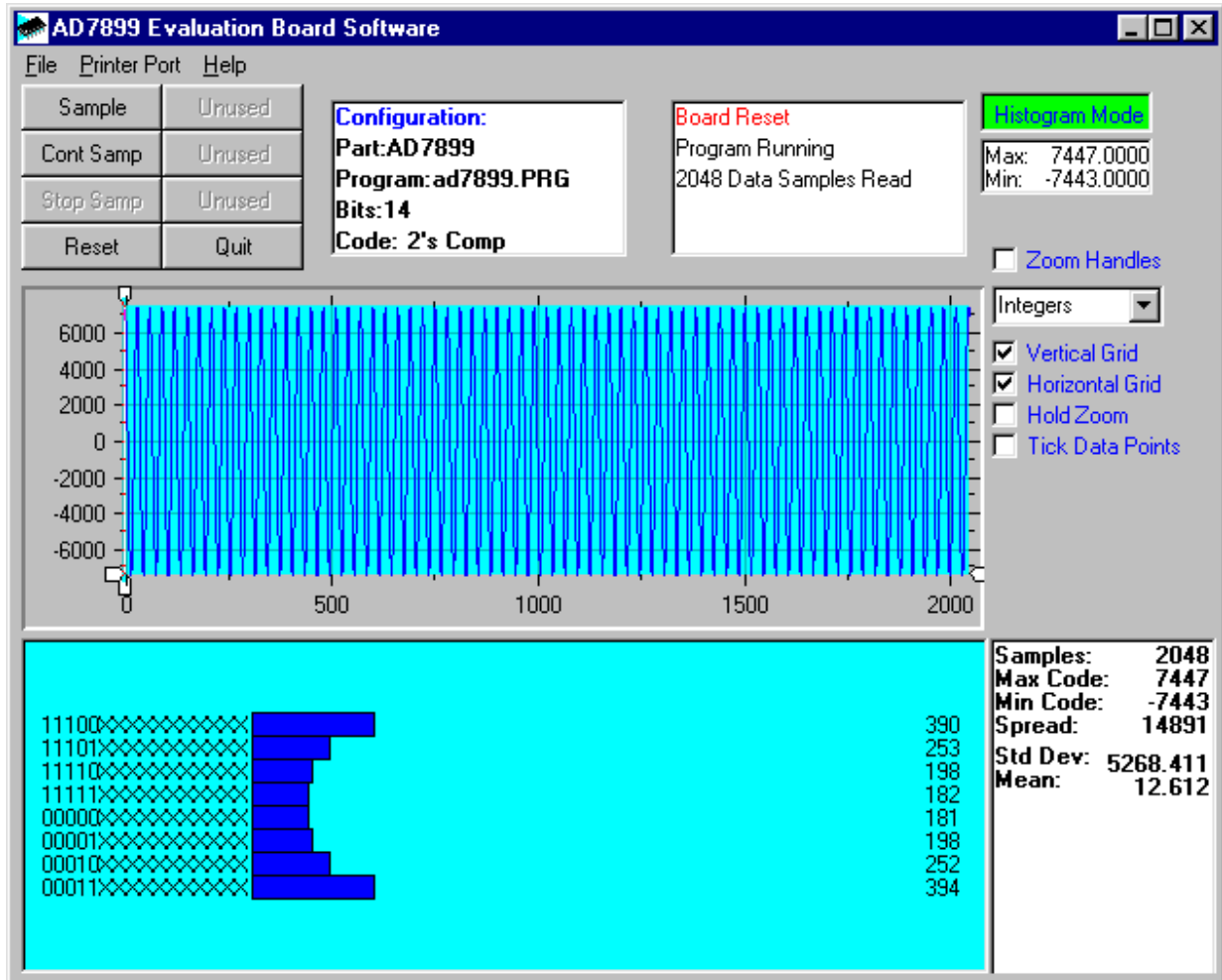
Figure 3. AD7899 Main Screen - Histogram Mode
