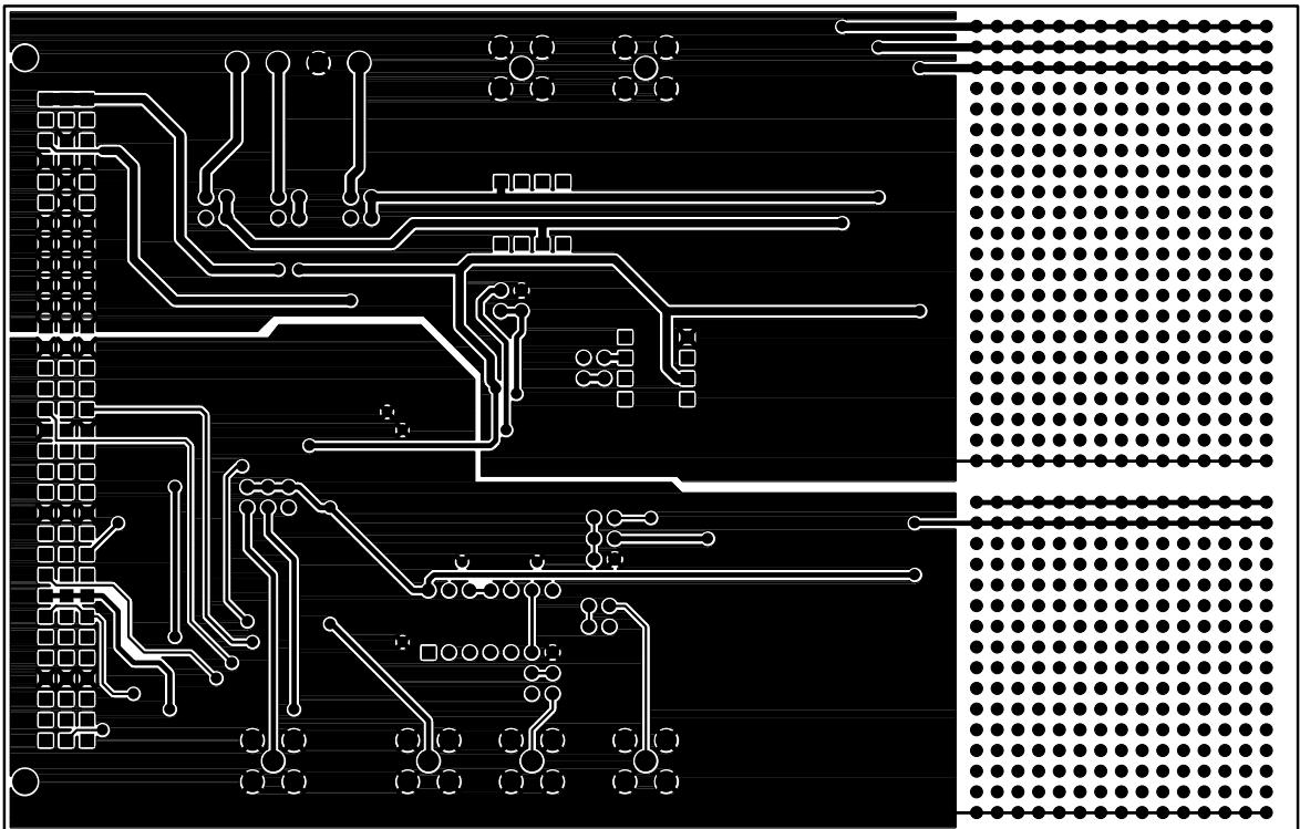
Figure 7. Solder Side Artwork.
