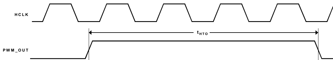
Figure 13. Timer PWM_OUT Cycle Timing
