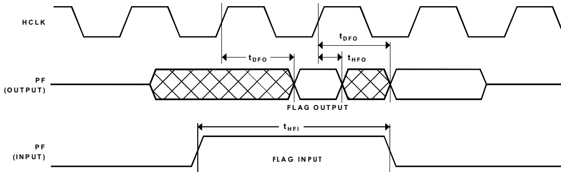
Figure 12. Programmable Flags Cycle Timing
