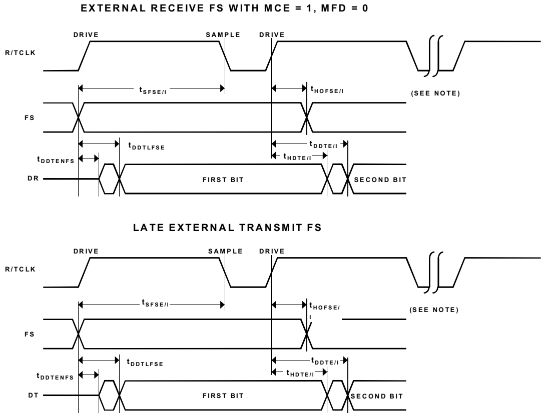
Figure 22. Serial Port (SPORT) Frame Synchronism
