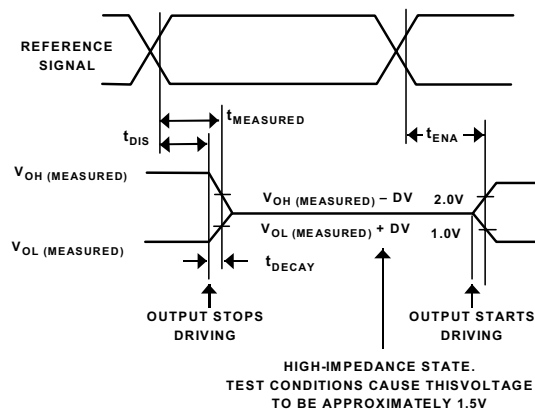
Figure 32. Output Enable/Disable
