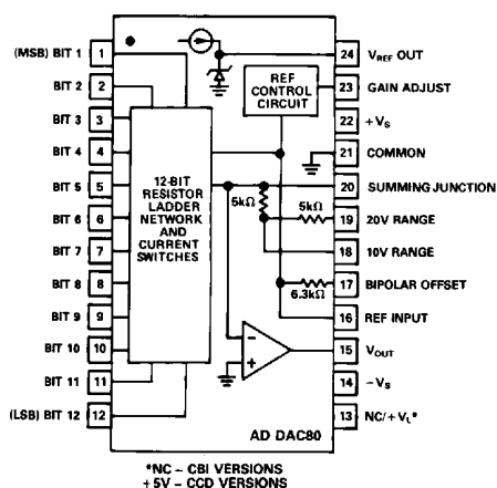
Voltage Model Functional Diagram and Pin Configuration
