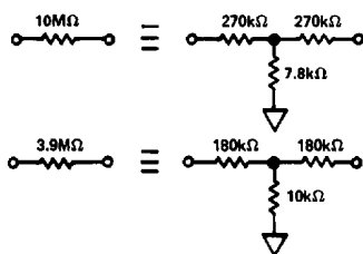
Figure 6. Equivalent Resistances
