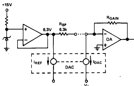
Figure 2. Bipolar Configuration
