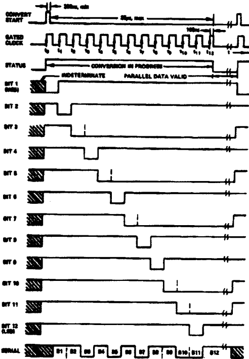
Figure 4. AD363-ADC Timing Diagram (Binary Code 110101011001)
