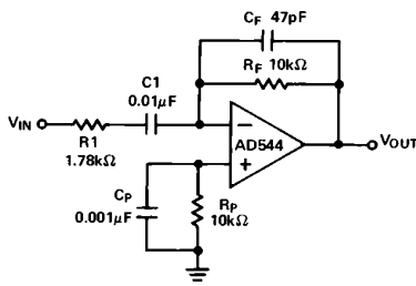
Figure 34. Differentiator
