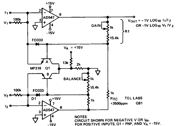
Figure 33. Log-Ratio Amplifier
