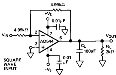
Figure 24a. Unity Gain Inverter
