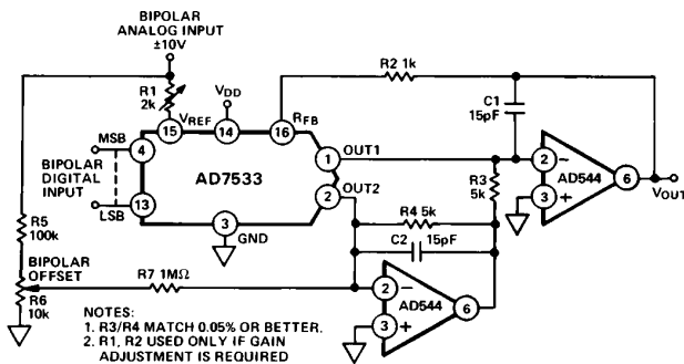
Figure 32a. AD544 Used as DAC Output Amplifiers
