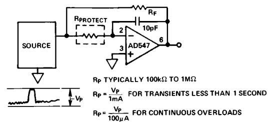
Figure 30. Input Protection
