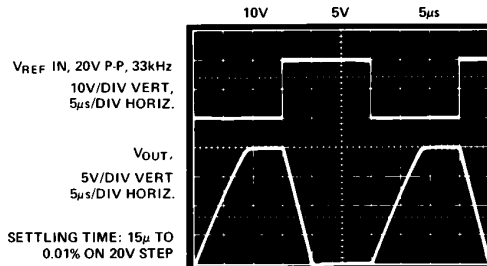
Figure 31b. Voltage Output DAC Settling Characteristic
