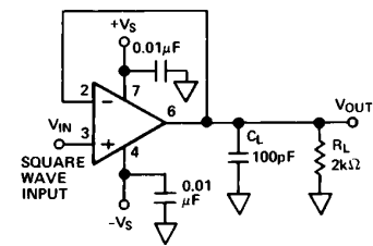
Figure 21c. Unity Gain Follower-AD542/AD547
