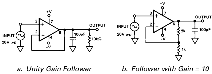
Figure 19. THD Test Circuits
