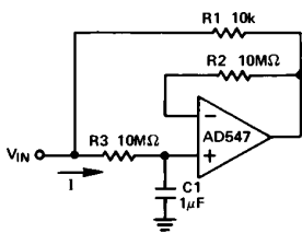
Figure 37. Capacitance Multiplier
