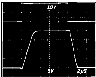
Figure 32b. Large Signal Response
