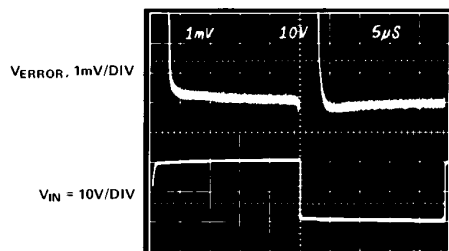
Figure 26. Settling Characteristic Detail-AD544
