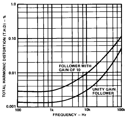
Figure 16. AD544 Total Harmonic Distortion vs. Frequency
