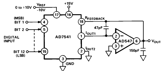
Figure 31a. AD547 Used as DAC Output Amplifier
