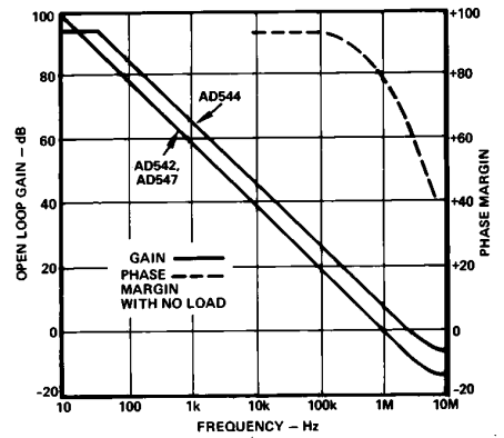
Figure 9. Open Loop Frequency Response
