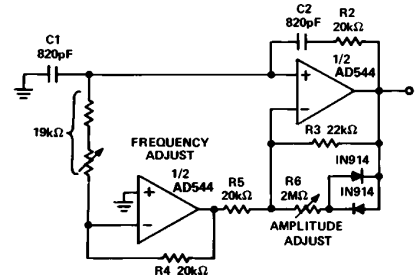
Figure 36. Wien-Bridge Oscillator- f_0 = 10 kHz
