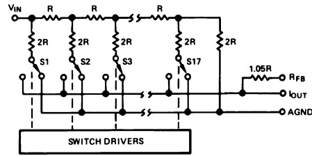
Figure 2. Simplified D/A Circuit of AD7118
