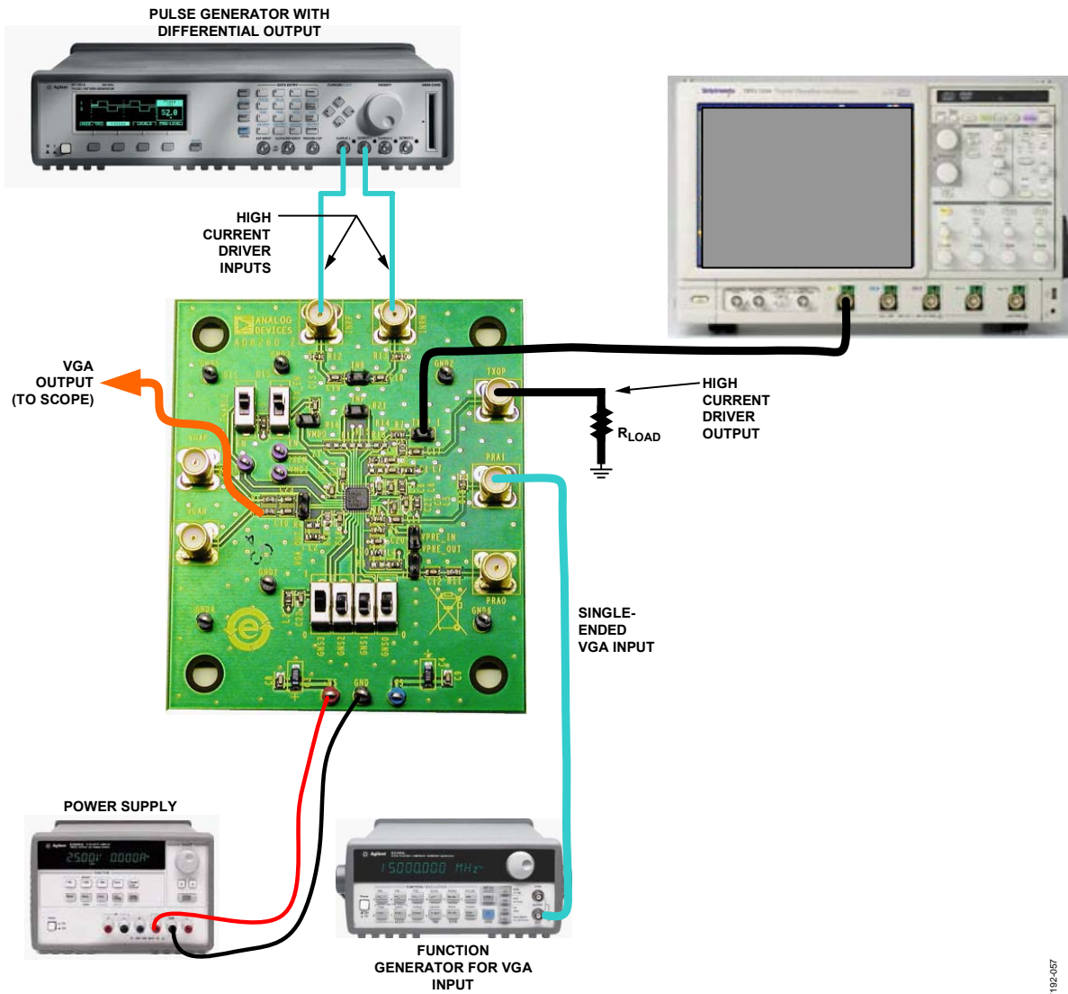
Figure 69. Typical Evaluation Board Connections
