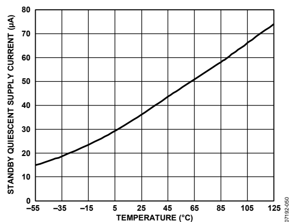
Figure 50. Standby Quiescent Supply Current vs. Temperature
