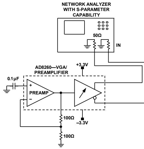
Figure 60. Test Circuit for Output Resistance of the VGA/Preamplifier
