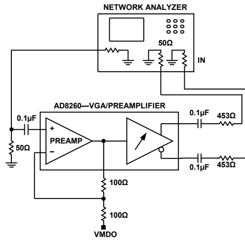
Figure 59. Test Circuit for Frequency Response and Group Delay of the VGA/Preamplifier
