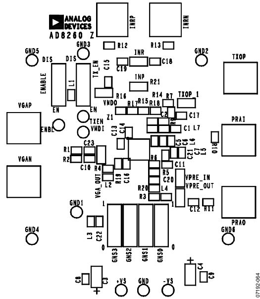
Figure 76. Component Side Silkscreen
