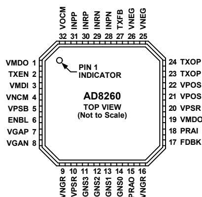
Figure 2. Pin Configuration
