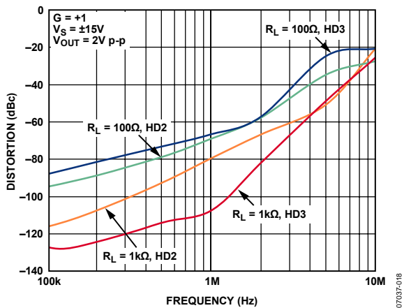
Figure 19. Harmonic Distortion vs. Frequency and Loads
