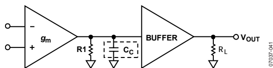
Figure 40. Topology
