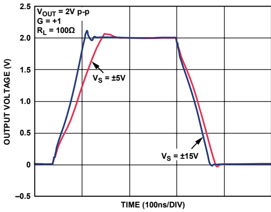
Figure 24. Large Signal Transient Response for Various Supply Voltages, R_L = 100\ \Omega
