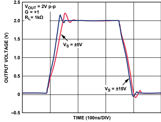
Figure 26. Large Signal Transient Response for Various Supply Voltages, R_L = 1\text{ k}\Omega
