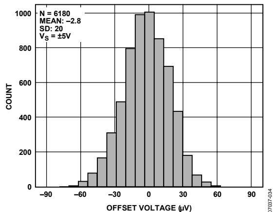
Figure 34. Input Offset Voltage Distribution, V_S = \pm 5V
