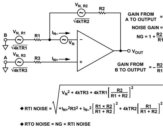
Figure 44. Op Amp Noise Analysis Model
