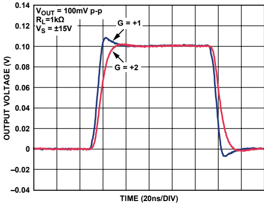
Figure 23. Small Signal Transient Response for Various Gains
