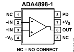
Figure 1. 8-Lead SOIC_N_EP (RD-8)
