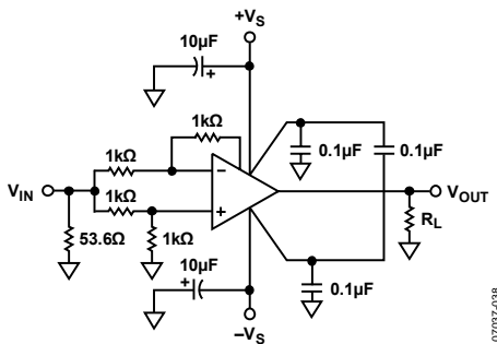
Figure 37. Common-Mode Rejection
