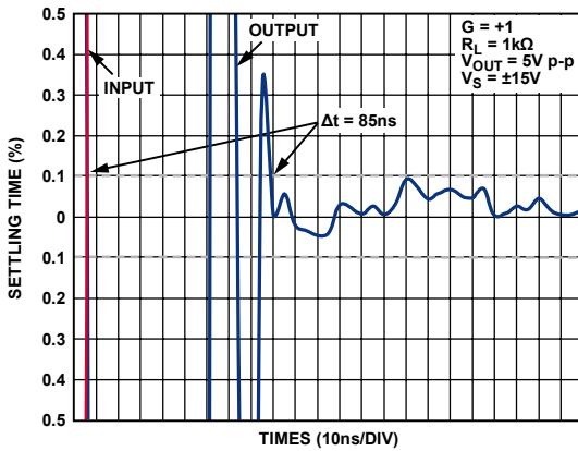
Figure 25. Settling Time
