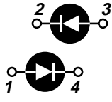
Anti-Parallel APT2X100D20J
