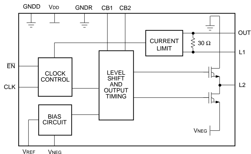
Figure 1. Block Diagram
