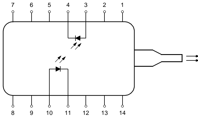
Figure 1. Pinout Schematic
