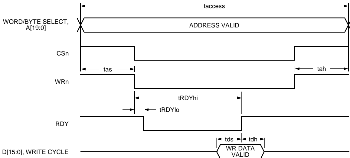
Microprocessor Access Write Cycle, Intel Protocol
