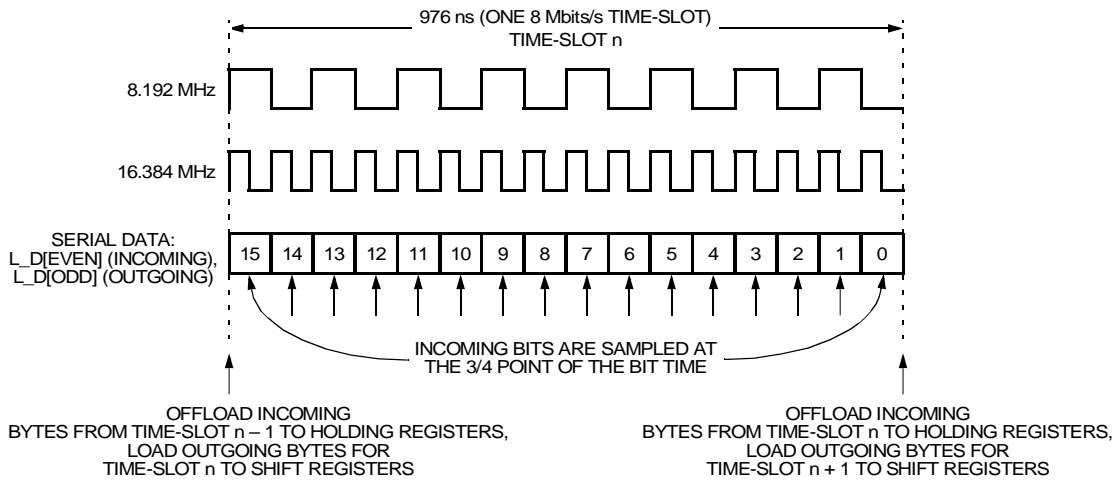
Figure 29. Local Stream 16.384 Mb/s Timing
