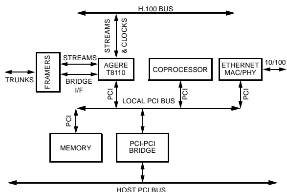
Figure 1. Basic Application of the T8110 as a CT Switch and CT-IP Payload Processor
