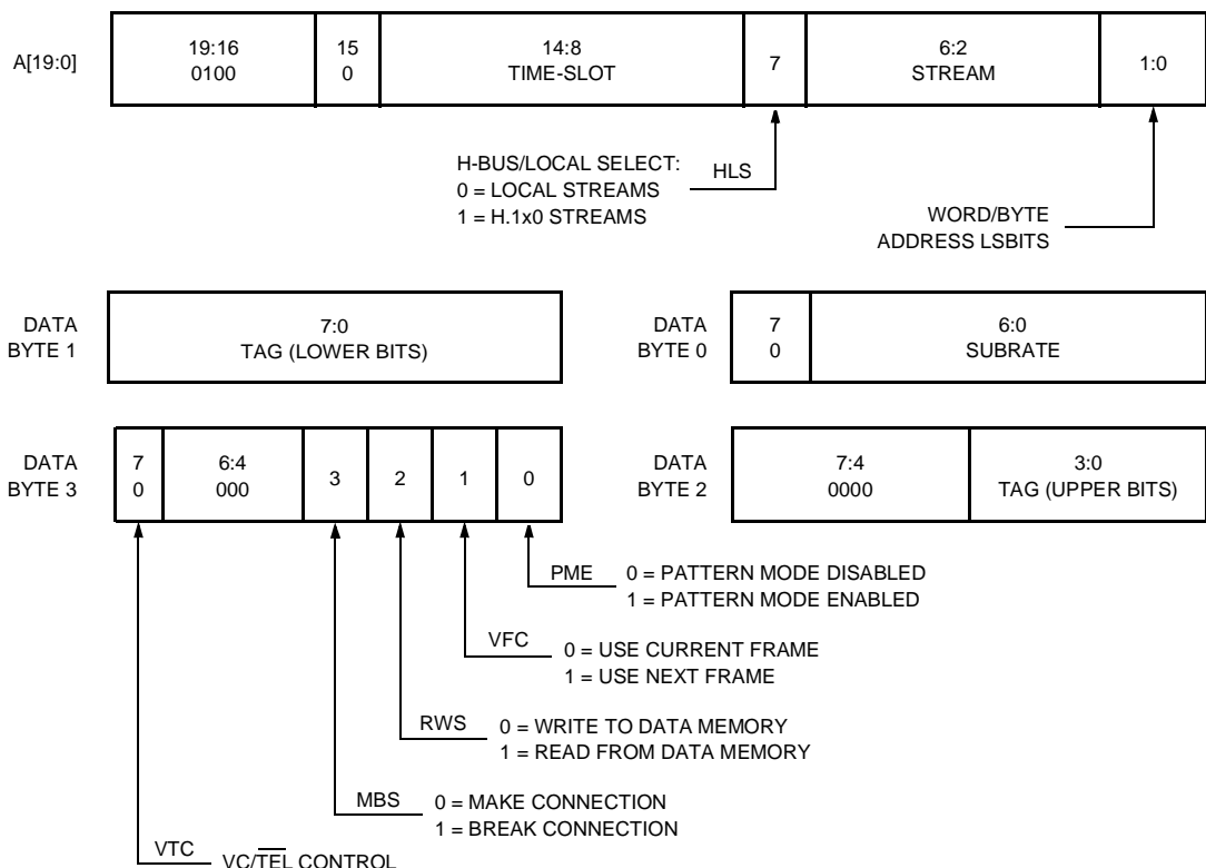
Figure 43. Microprocessor Programming—Make/Break/Query Telephony Connections
