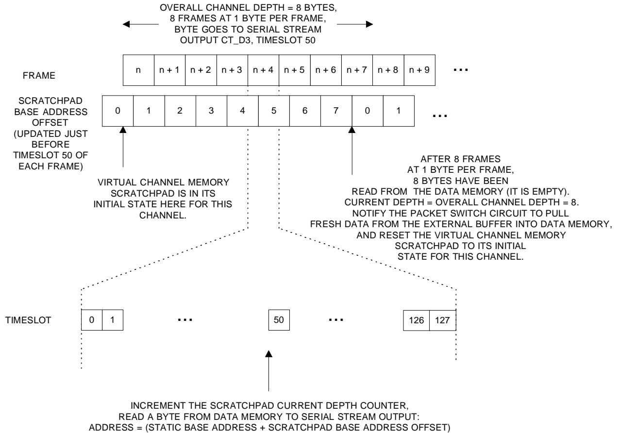
Figure 54. Nonbonded Virtual Channel in the PULL Direction
