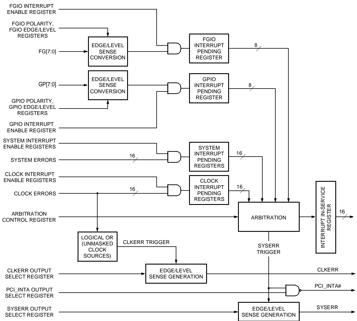
Figure 34. Interrupt Controller
