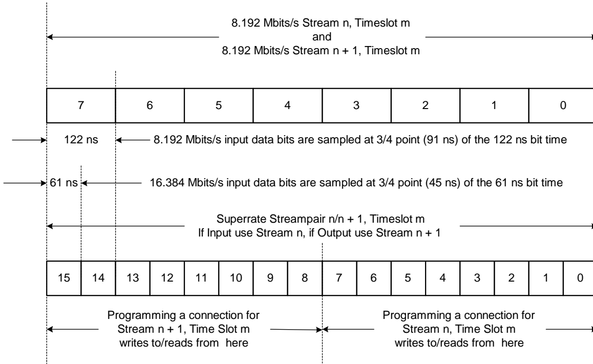
Figure 32. Relationship Between 8.192 Mbits/s and 16.384 Mbits/s Time-Slots
