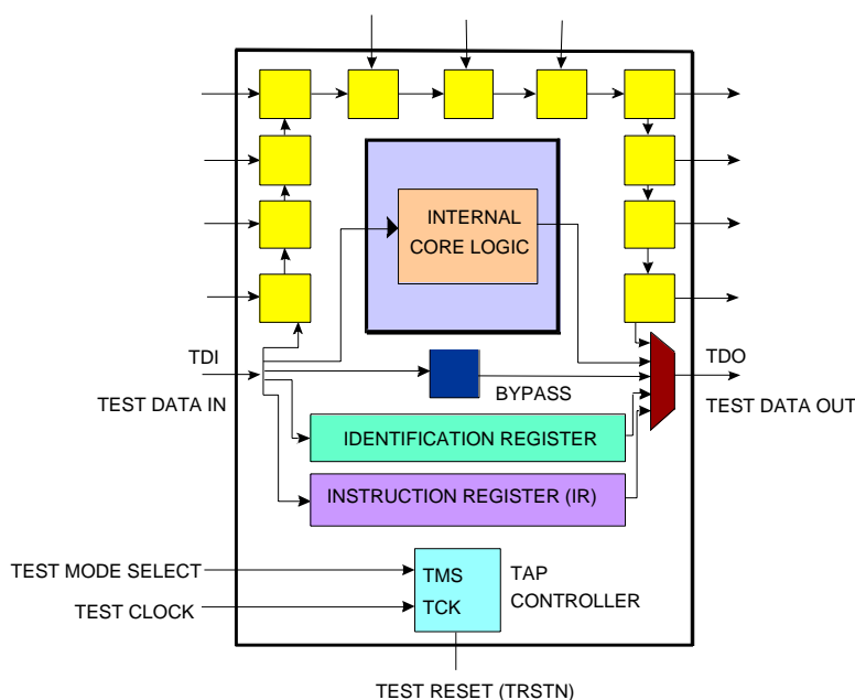
Figure 65. IEEE* 1149.1 Boundary-Scan Architecture
