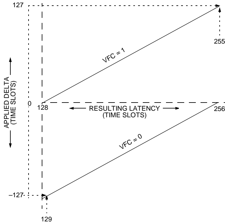
Figure 66. Constant Delay Connection Latency
