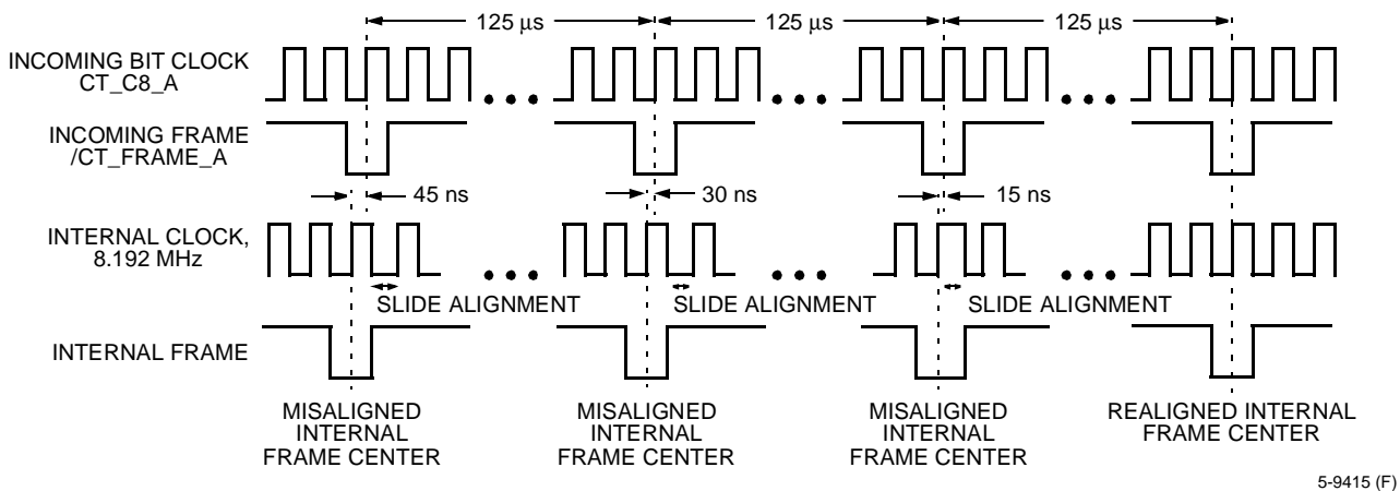
B. Phase Alignment—SLIDE
