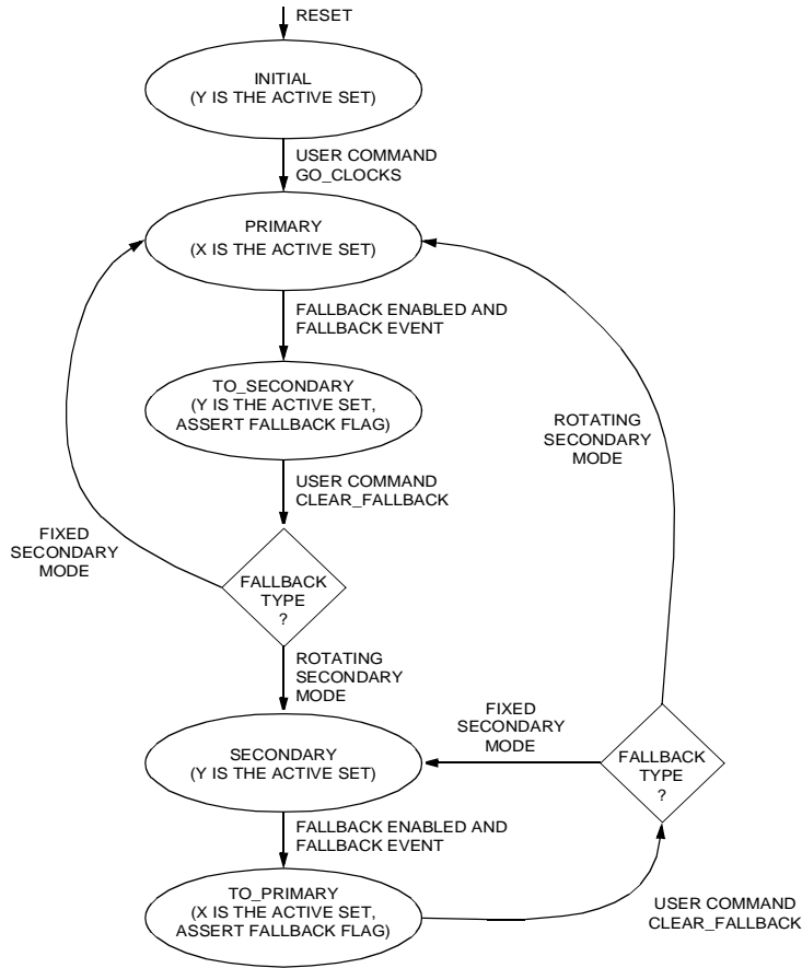
Figure 23. T8110 Clock Fallback States
