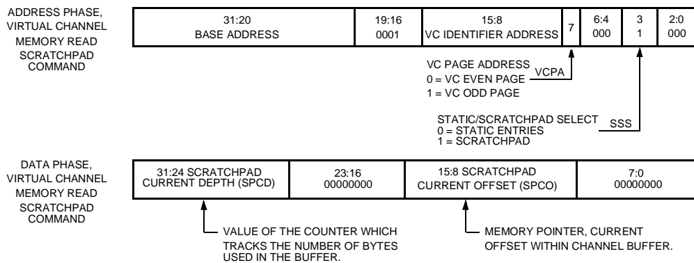
Figure 41. PCI Programming—Read Virtual Channel Scratchpad Command
