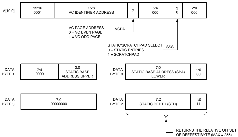
Figure 47. Microprocessor Programming—Read Virtual Channel Static Command
