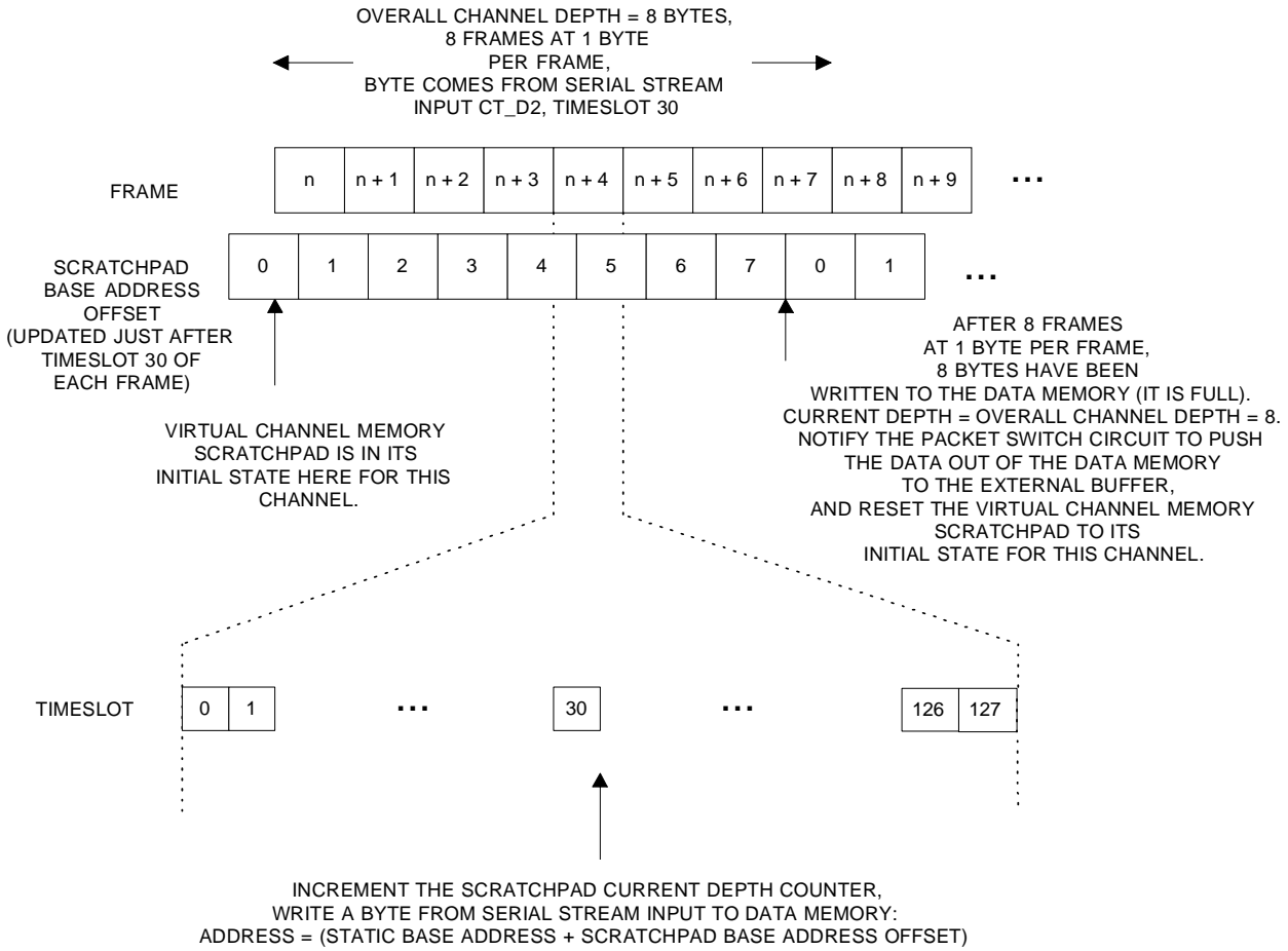
Figure 53. Nonbonded Virtual Channel in the PUSH Direction
