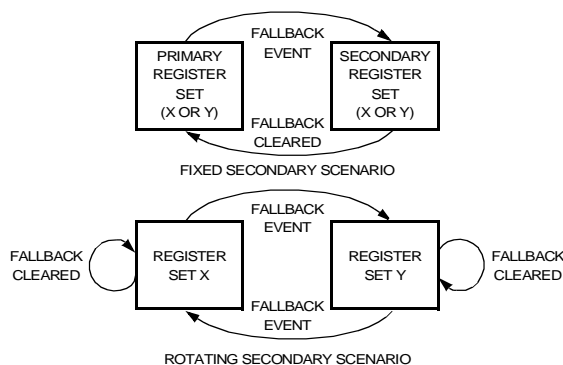
Figure 22. Fallback—Fixed vs. Rotating Secondary
