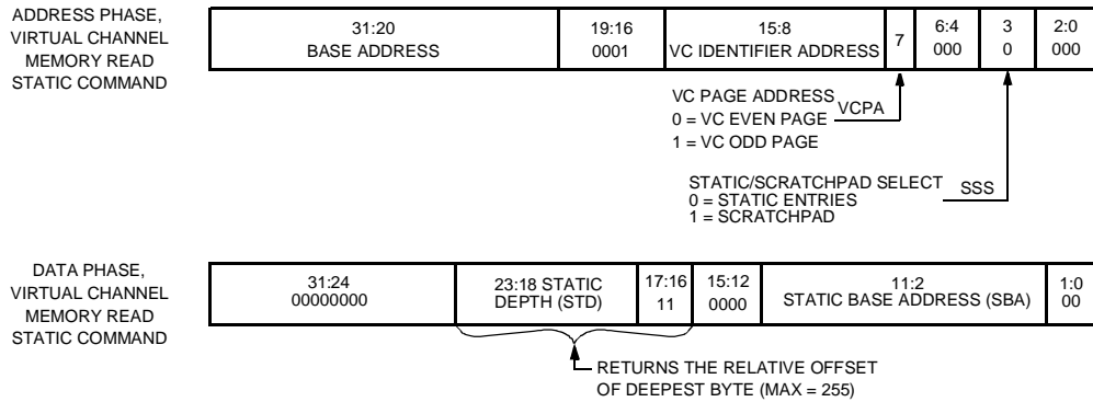
Figure 40. PCI Programming—Read Virtual Channel Static Command
