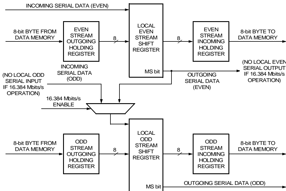
Figure 30. Local Stream 16.384 Mb/s Circuit
