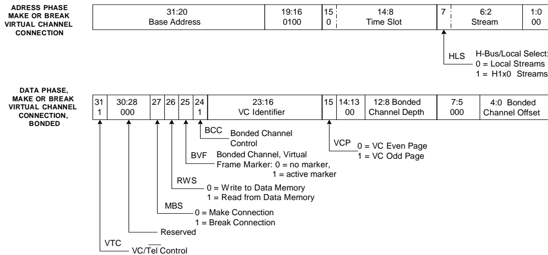
Figure 38. PCI Programming—Make/Break/Query Virtual Channel Bonded Connection
