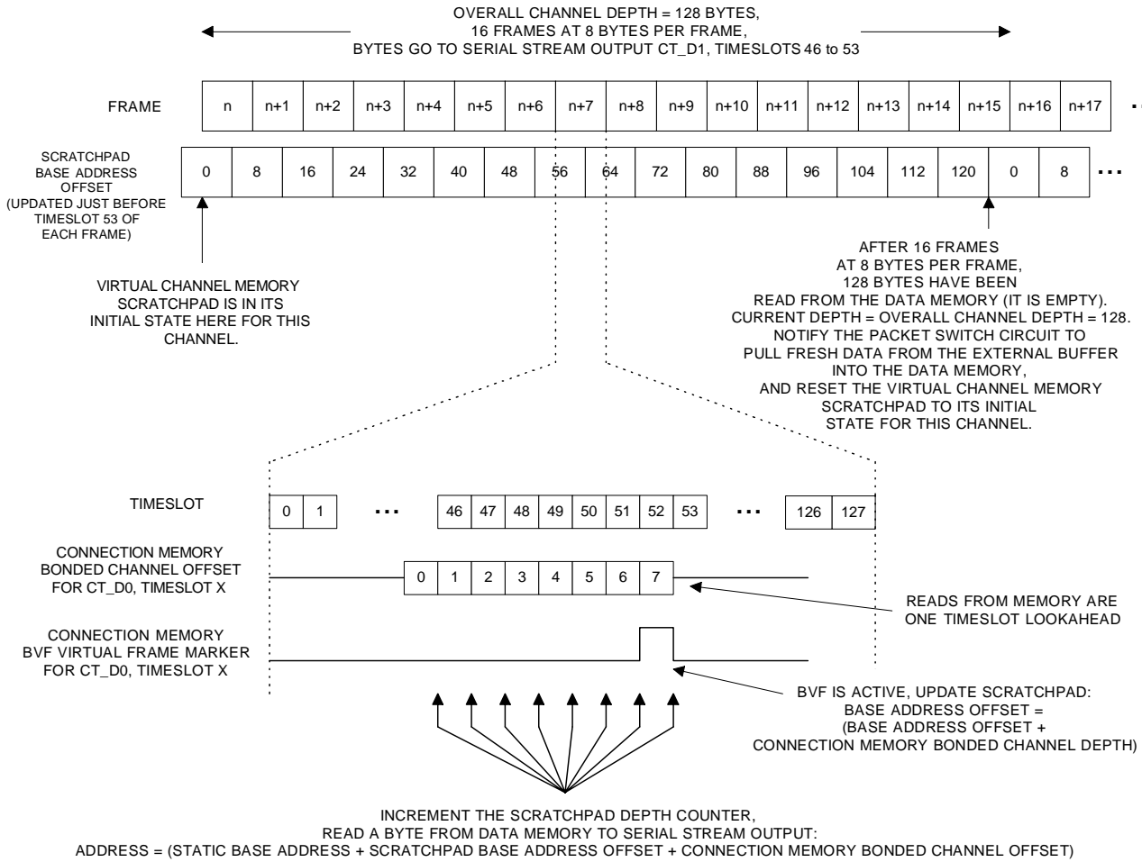
Figure 57. Bonded Virtual Channel in the PULL Direction
