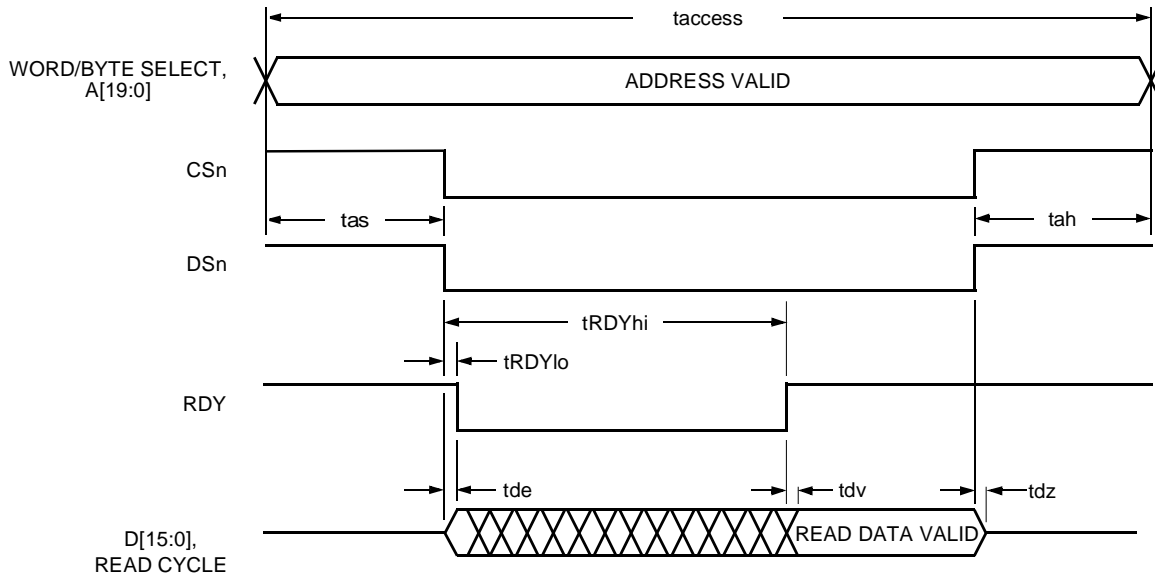
Microprocessor Access Read Cycle, Intel Protocol
