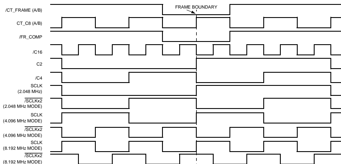
Figure 59. Clock Alignment
