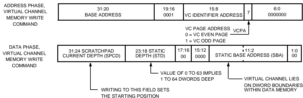
Figure 39. PCI Programming—Write Virtual Channel Command
