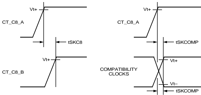
Figure 61. Detailed Clock Skew Timing Diagram
