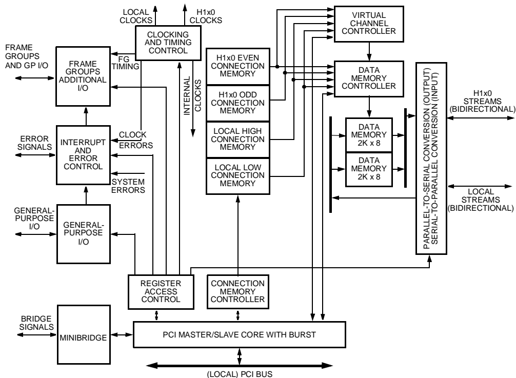
Figure 3. T8110 Block Diagram
