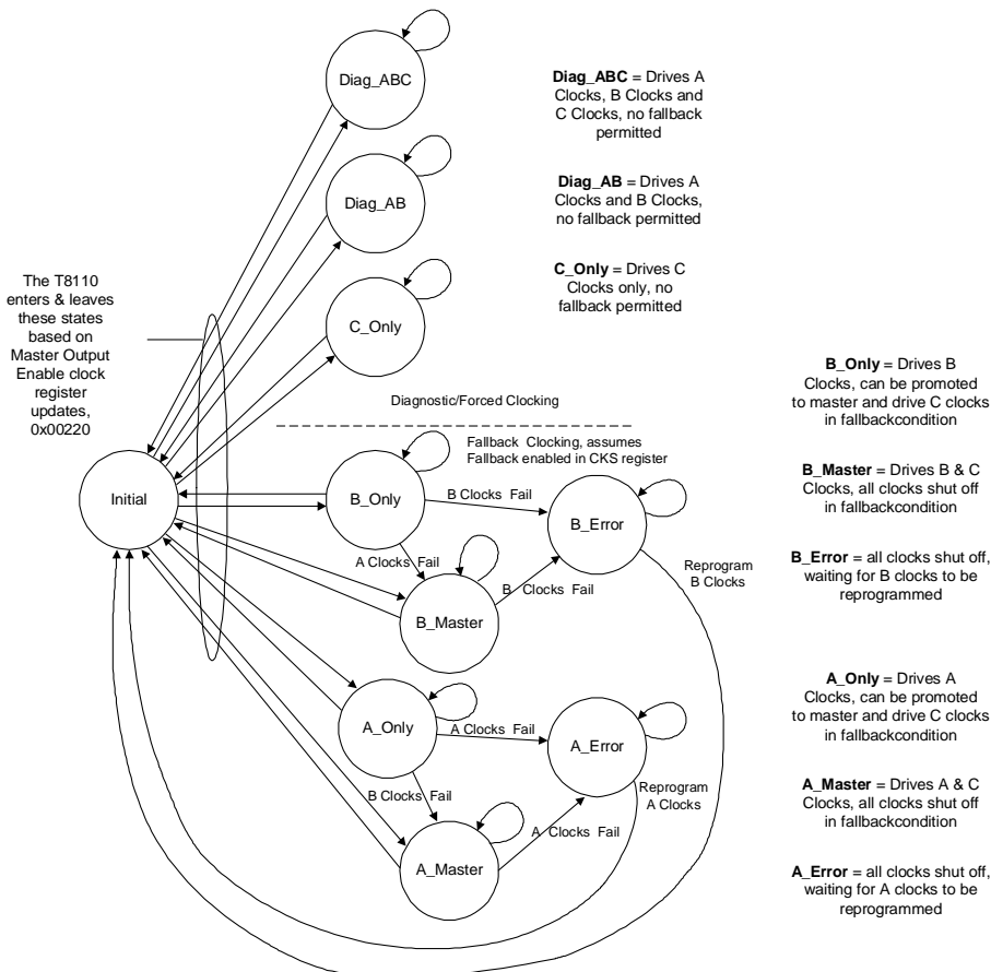
Figure 24. T8110 H-Bus Clock Enable States
