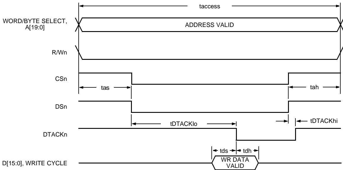
Figure 18. Microprocessor Access Timing, Motorola Protocol
