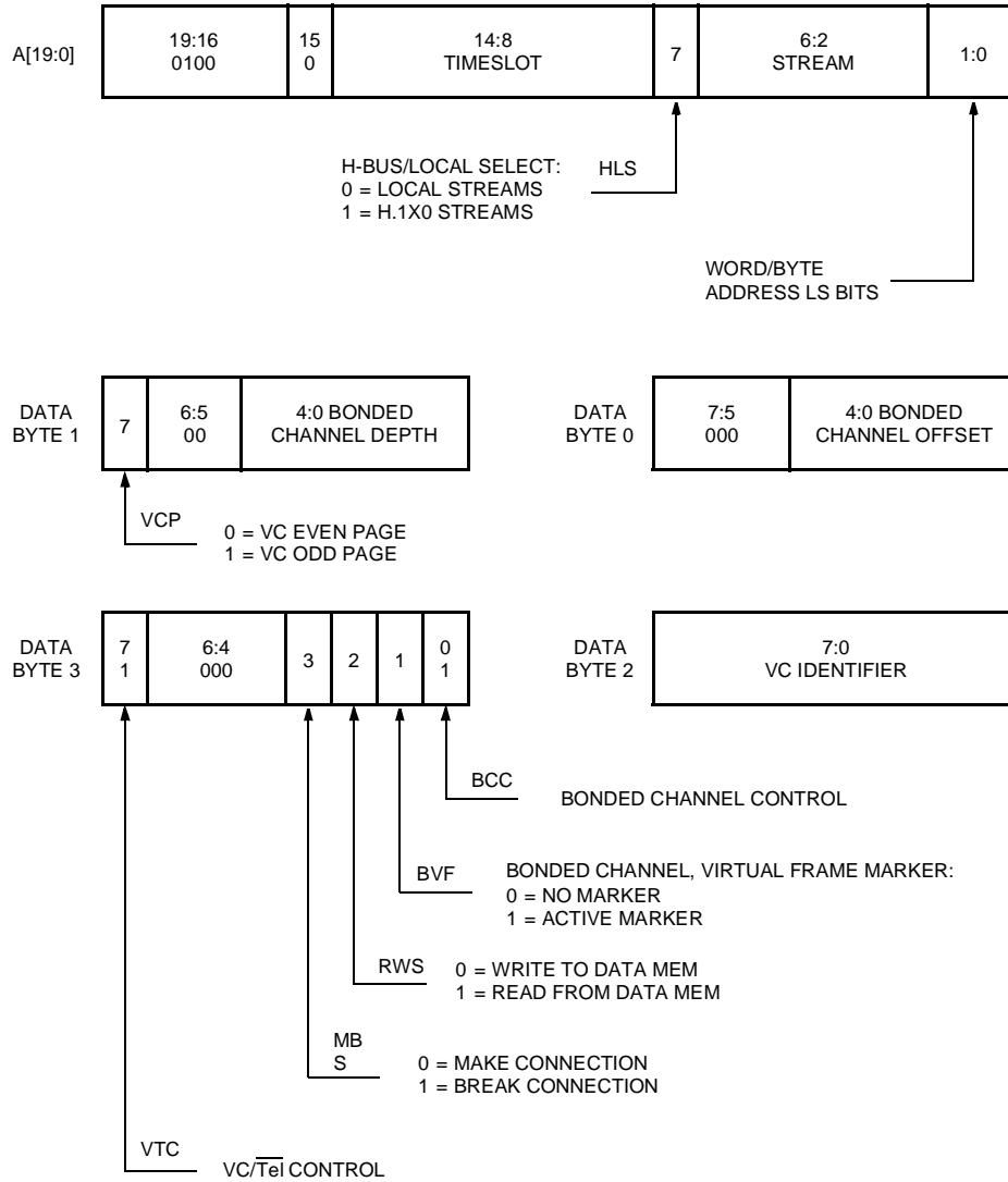
Figure 45. Microprocessor Programming—Make/Break/Query Virtual Channel Bonded Connection
