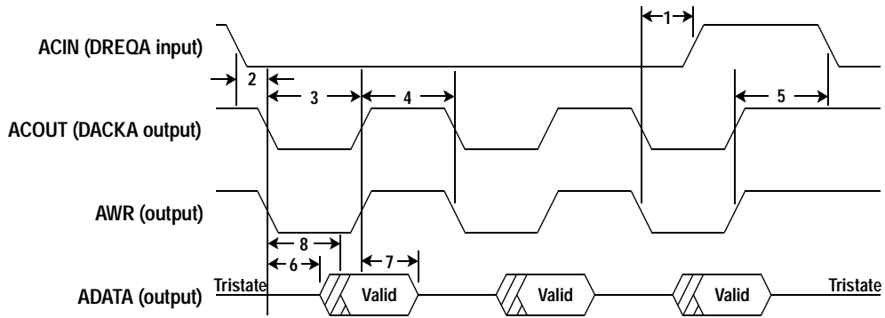
Figure 11: Port A Burst Write Timing, Slave Mode
