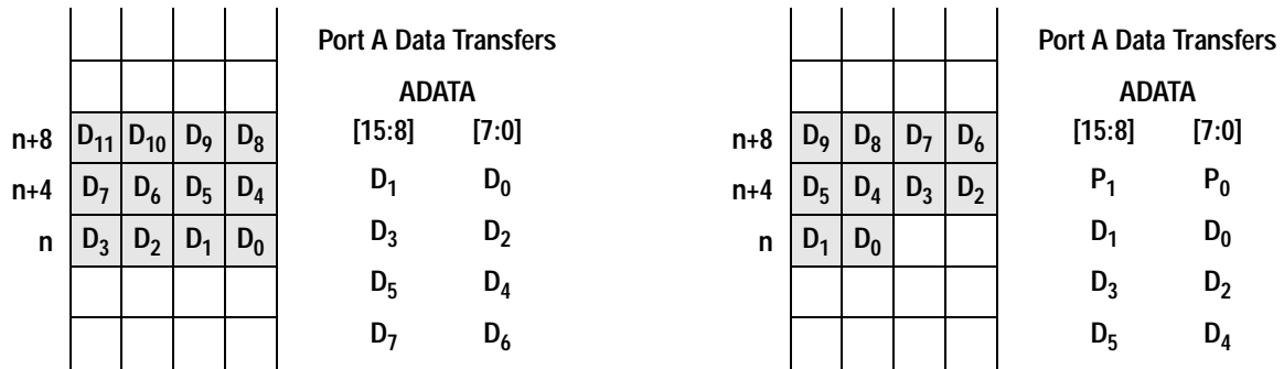
Part (a): Zero Bytes of Padding
