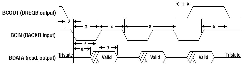
Figure 13: Port B Burst Read Timing, Master Mode
