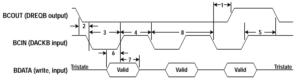
Figure 14: Port B Burst Write Timing, Master Mode
