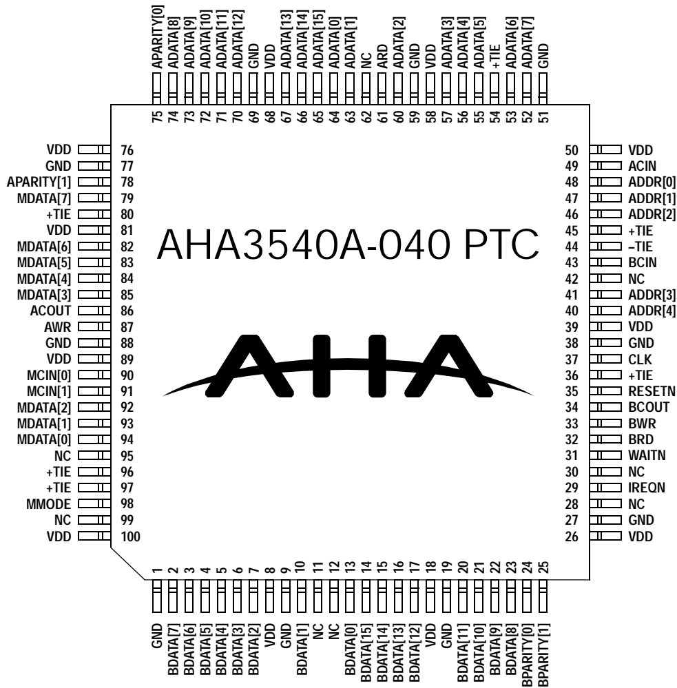
Figure 4: TQFP Pinout
