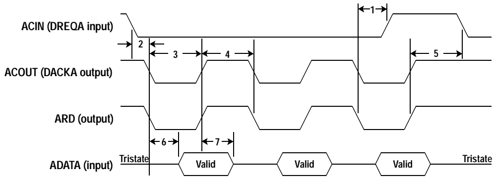
Figure 12: Port A Burst Read Timing, Slave Mode
