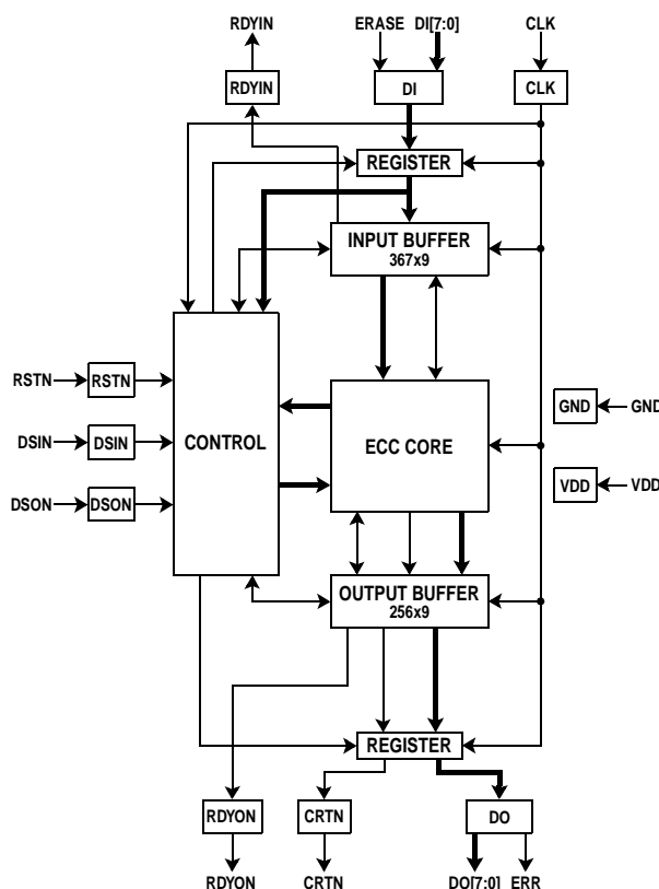
Figure 1: Block Diagram
