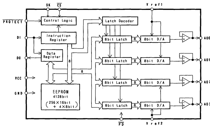
Block Diagram
