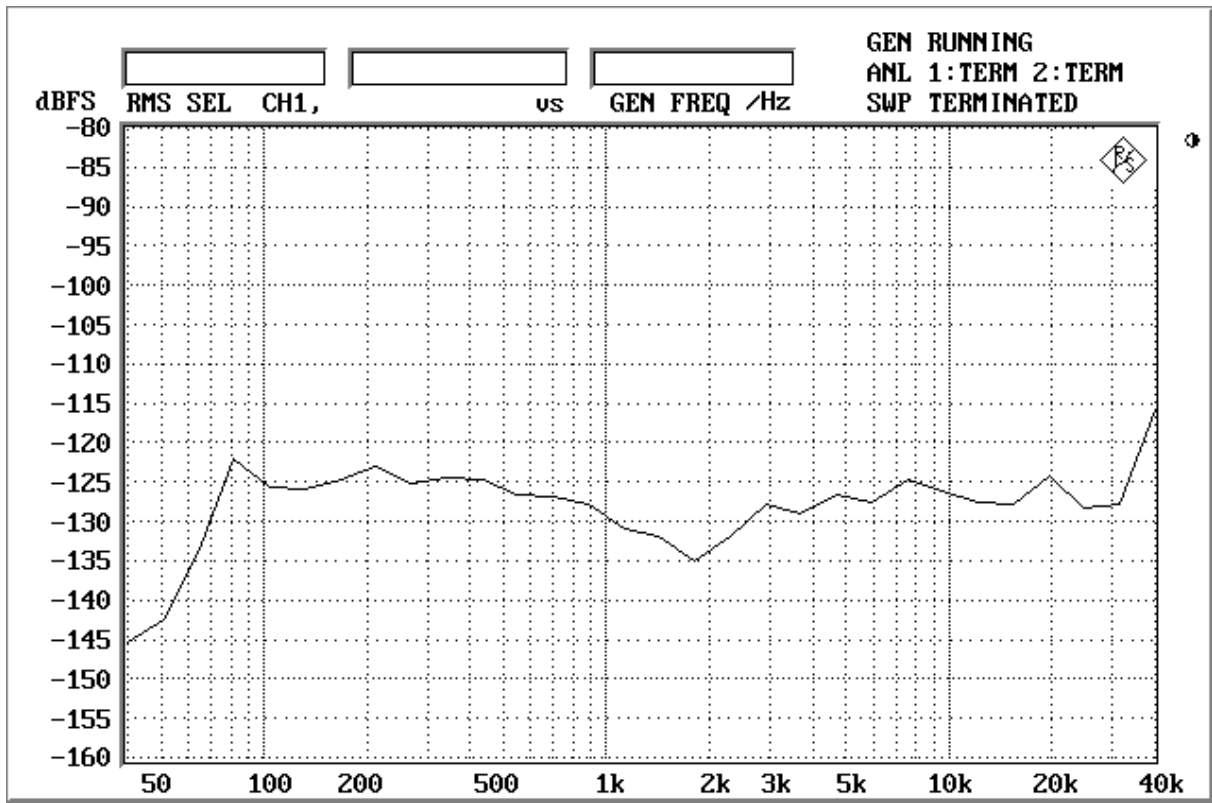
Fig.18 Crosstalk
