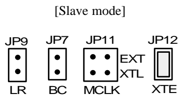
Figure 2. Jumper set up (D/A)
