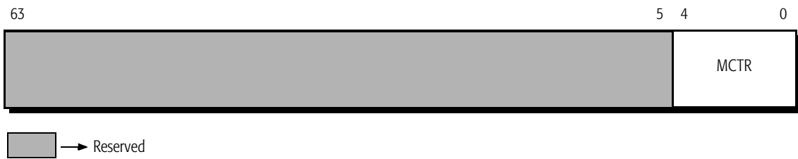
Figure 29. Machine-Check Type Register (MCTR)
