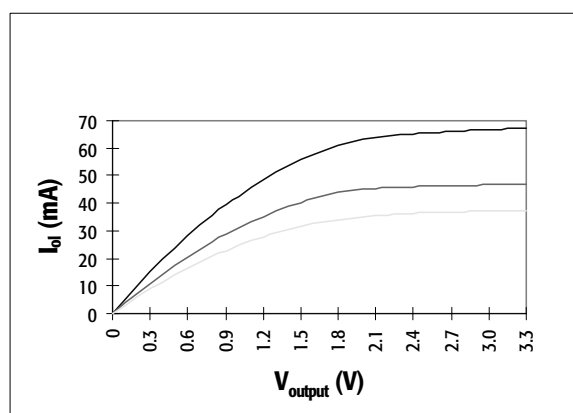
Figure 80. K6STD Pulldown V/I Curves
