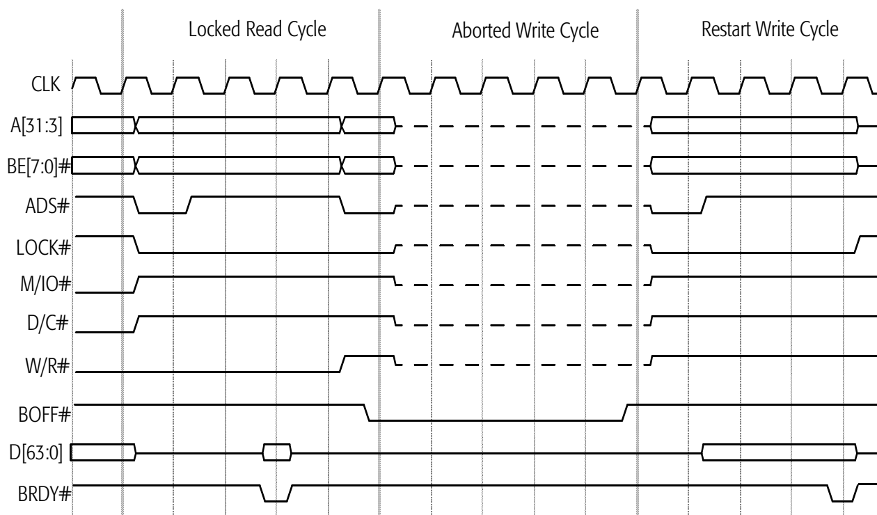
Figure 60. Locked Operation with BOPF# Intervention
