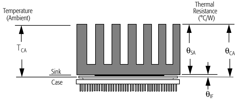
Figure 91. Thermal Model
