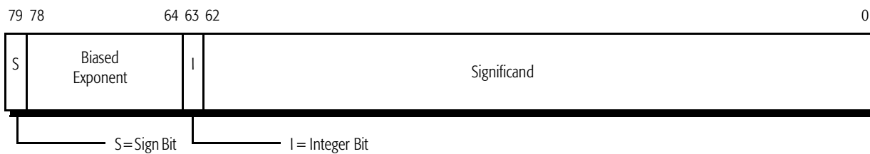
Figure 15. Precision Real Data Types
