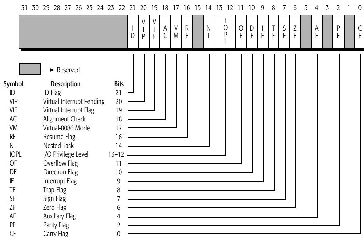
Figure 18. EFLAGS Registers
