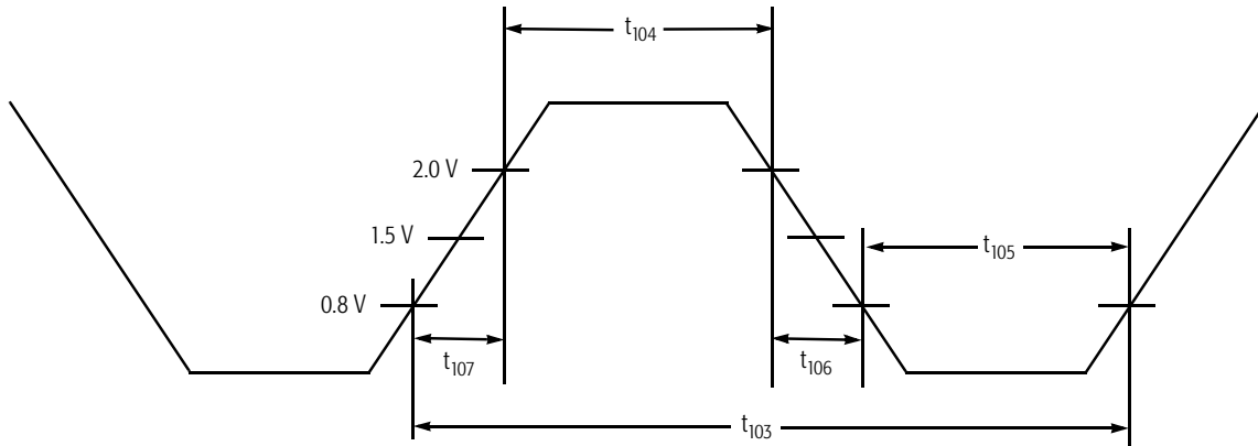
Figure 88. TCK Waveform
