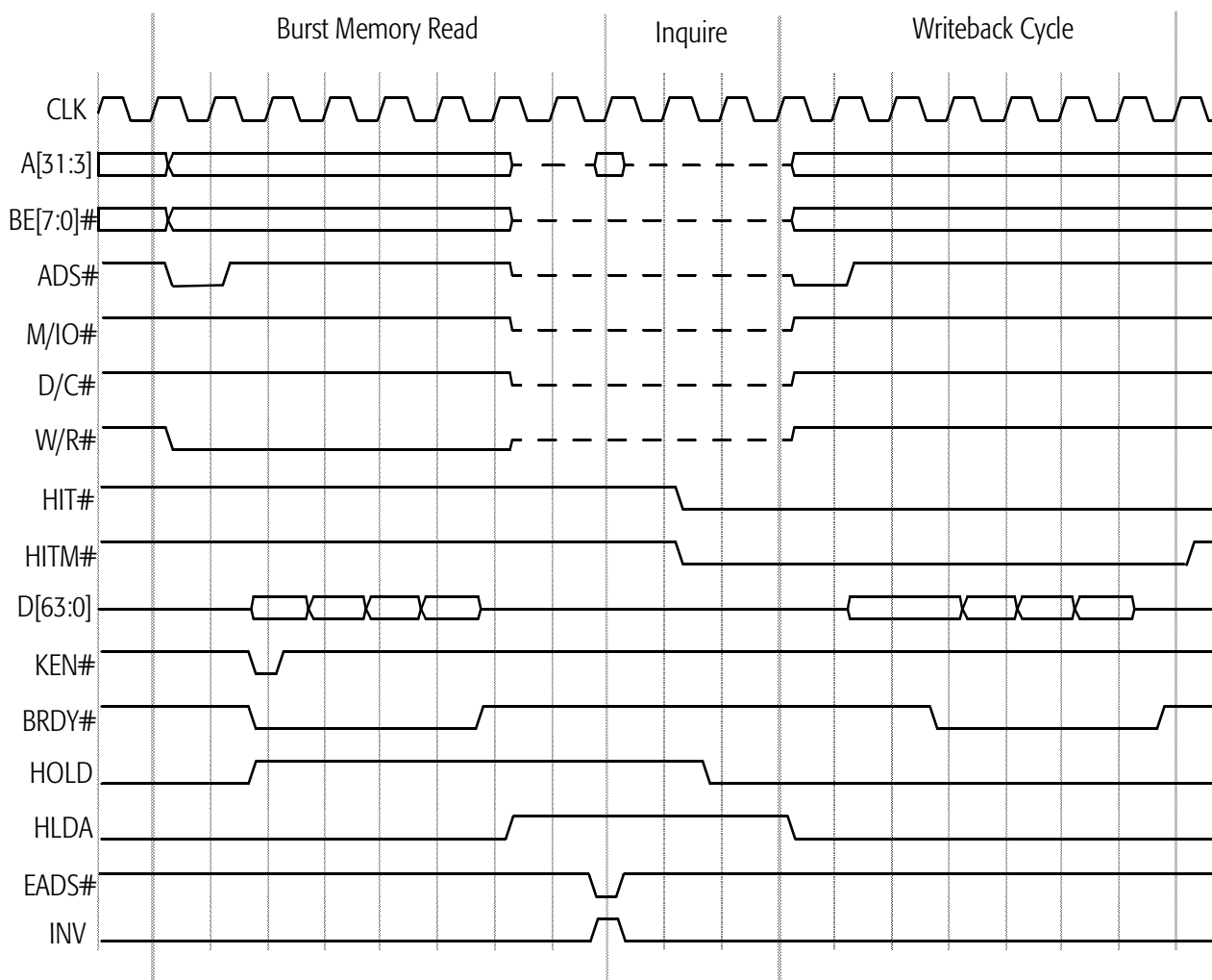
Figure 53. HOLD-Initiated Inquire Hit to Modified Line
