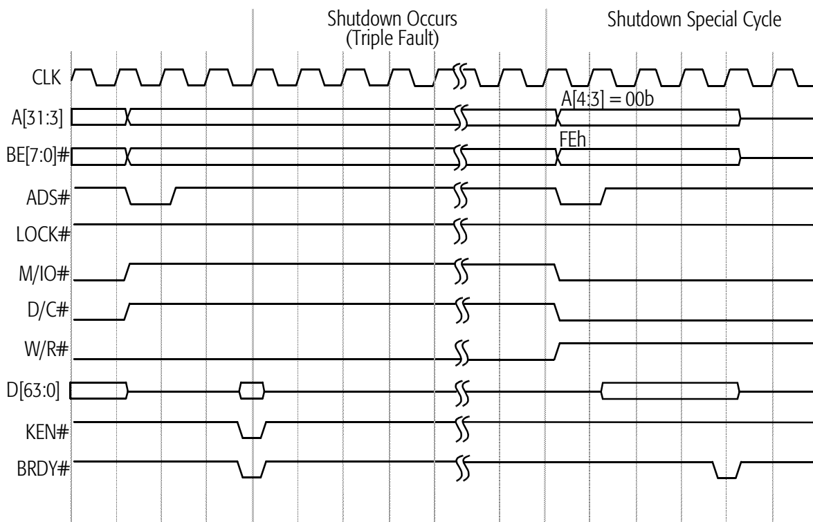
Figure 63. Shutdown Cycle
