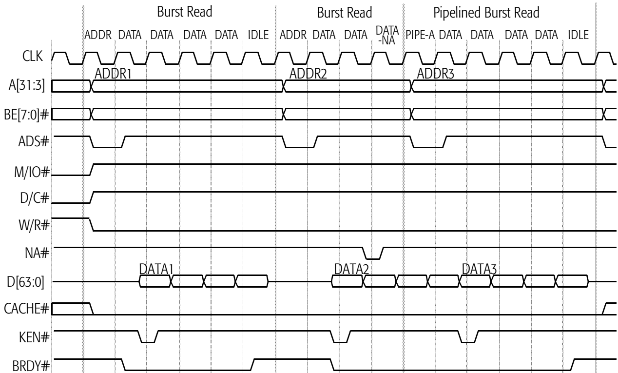
Figure 47. Burst Reads and Pipelined Burst Reads
