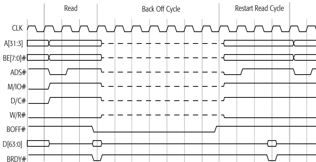
Figure 58. BOFF# Timing
