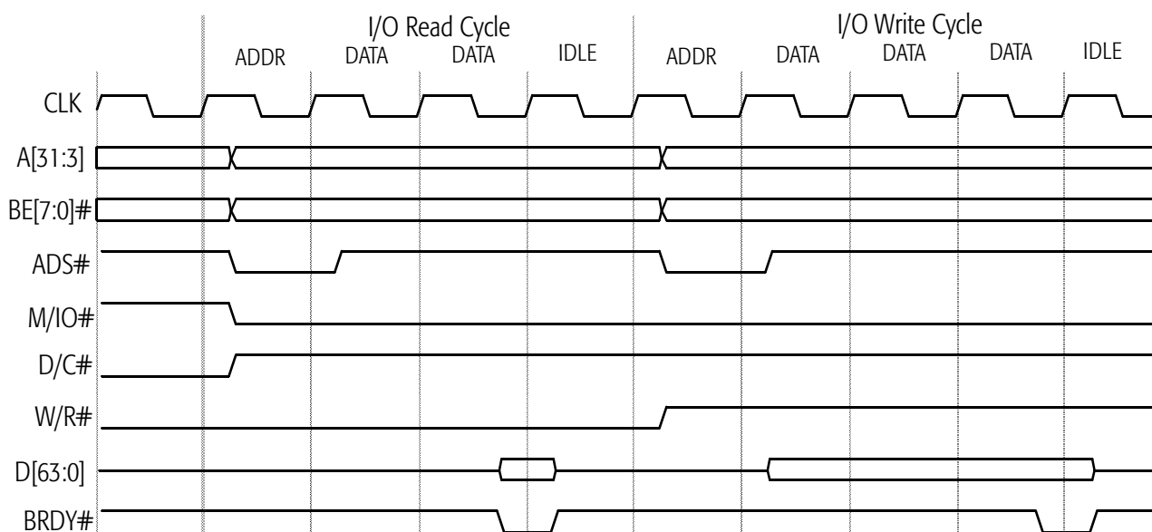
Figure 49. Basic I/O Read and Write
