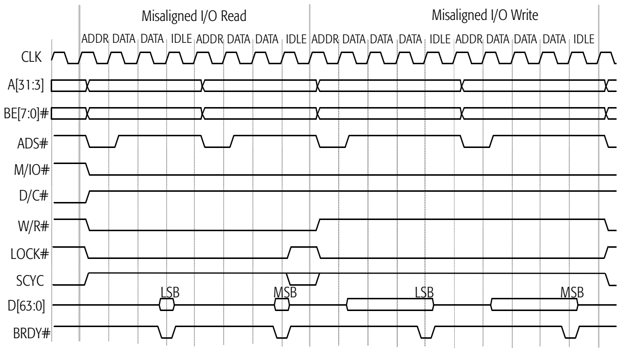
Figure 50. Misaligned I/O Transfer
