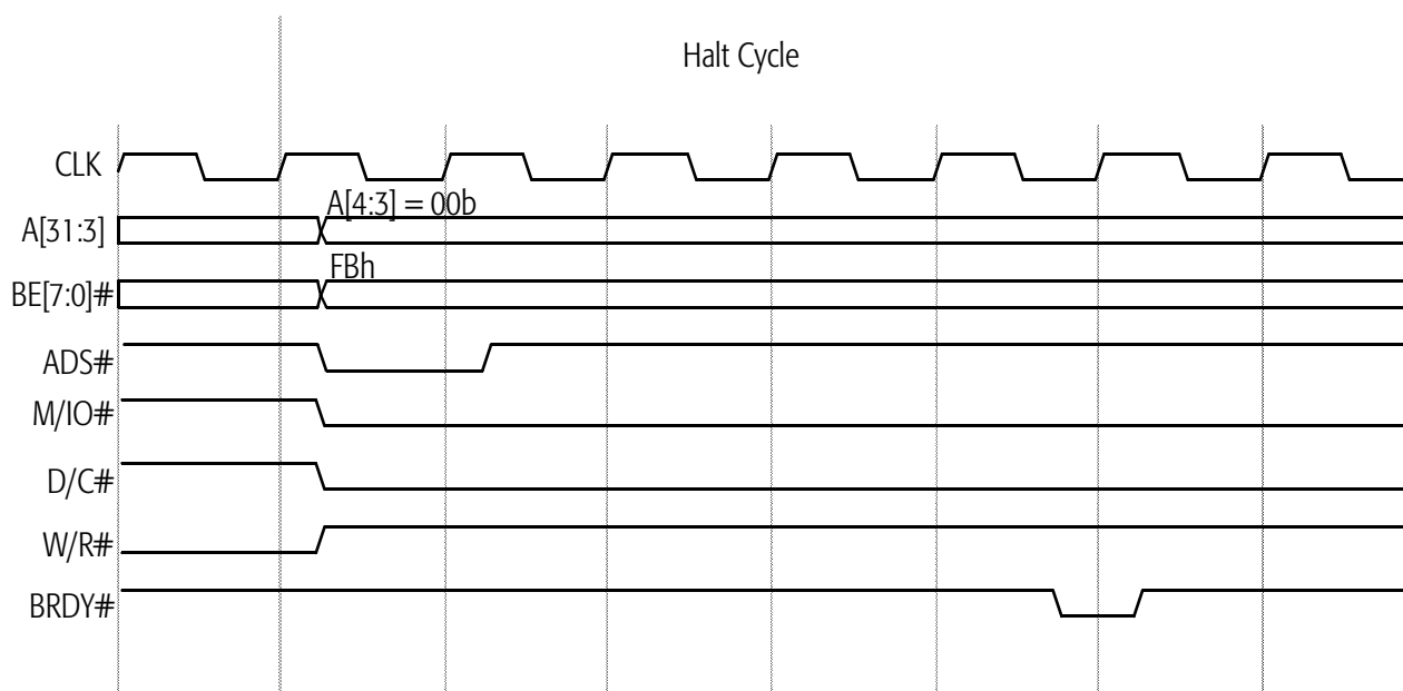
Figure 62. Basic Special Bus Cycle (Halt Cycle)
