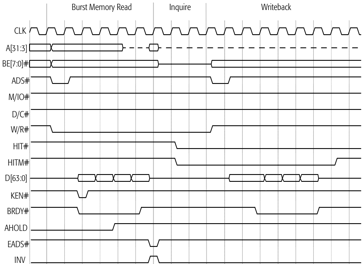
Figure 56. AHOLD-Initiated Inquire Hit to Modified Line
