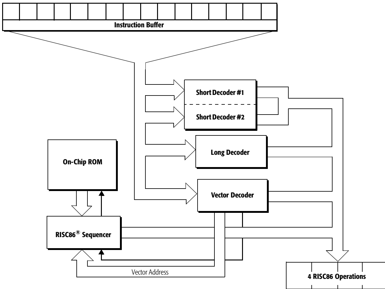
Figure 4. AMD-K6 ® Processor Decode Logic
