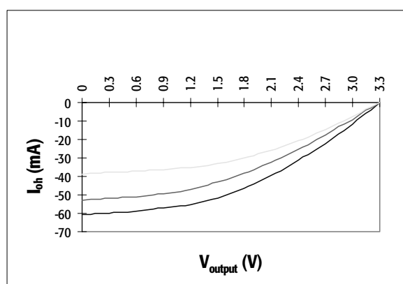
Figure 81. K6STD Pullup V/I Curves
