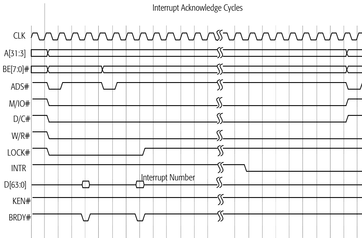
Figure 61. Interrupt Acknowledge Operation
