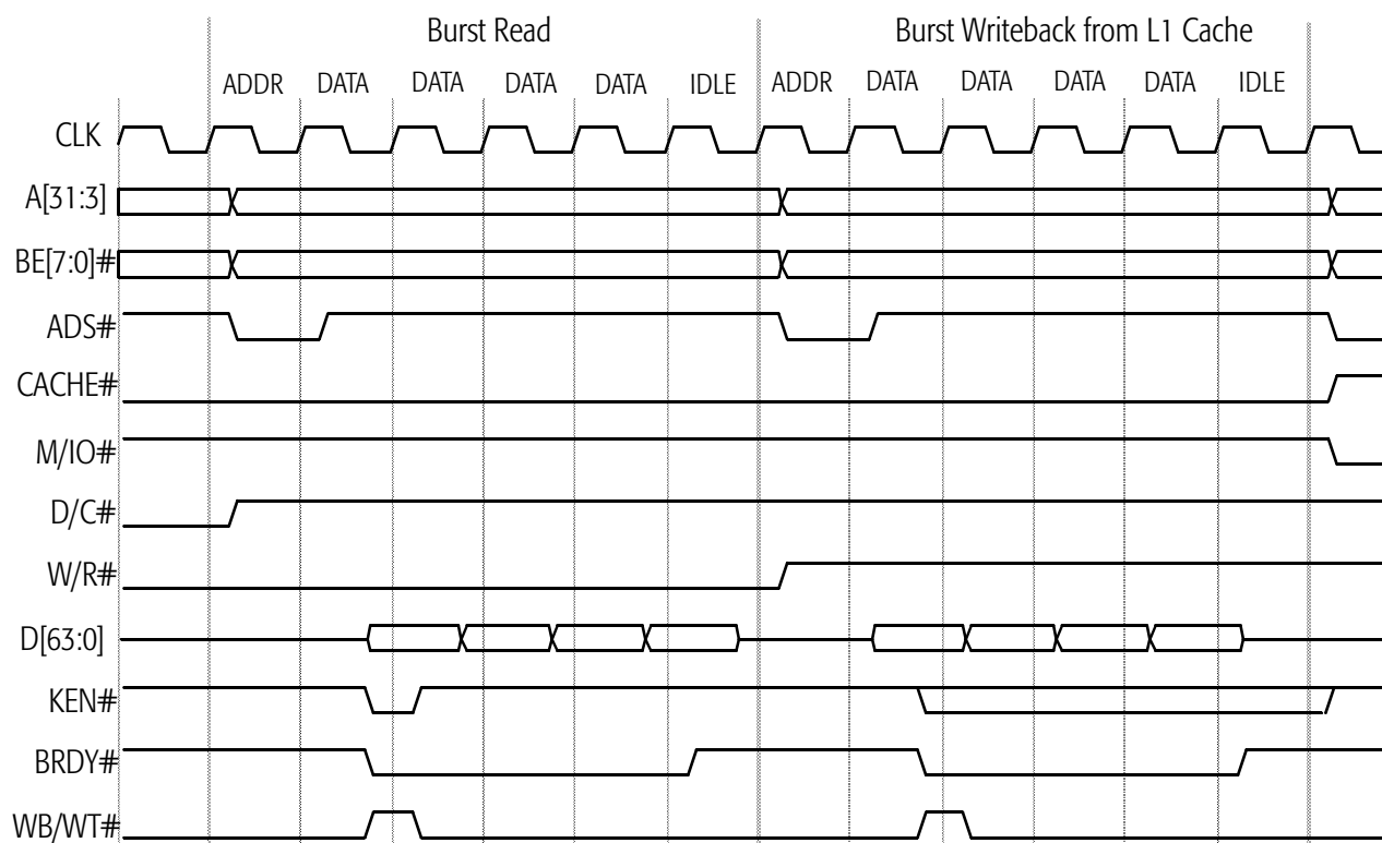
Figure 48. Burst Writeback due to Cache-Line Replacement
