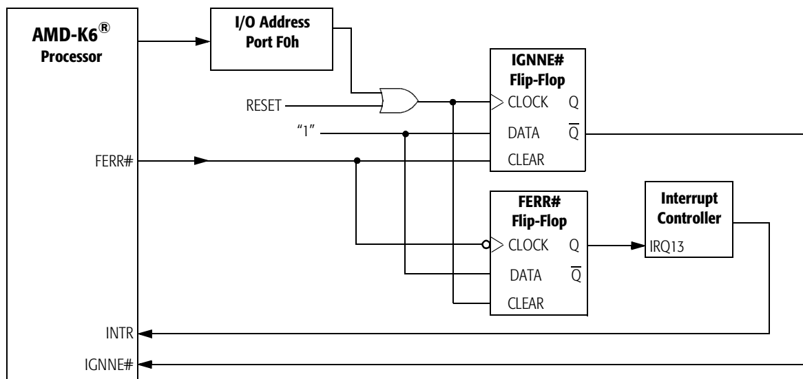
Figure 71. External Logic for Supporting Floating-Point Exceptions
