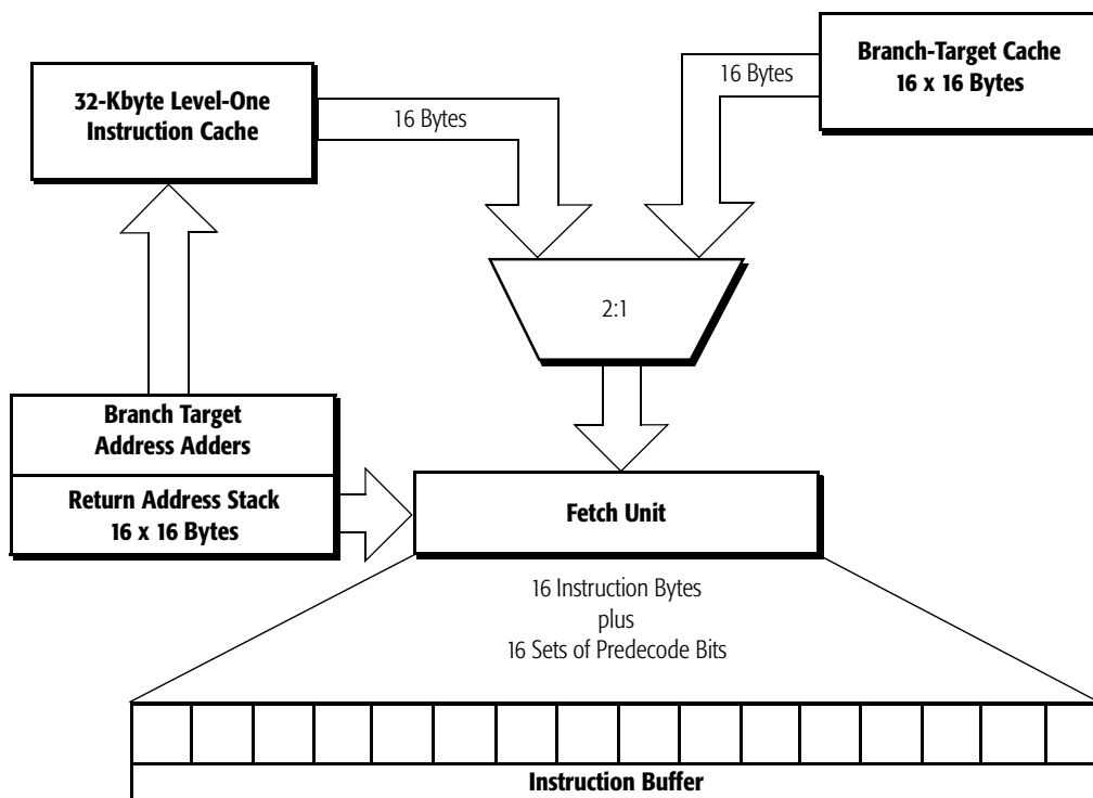
Figure 3. The Instruction Buffer
