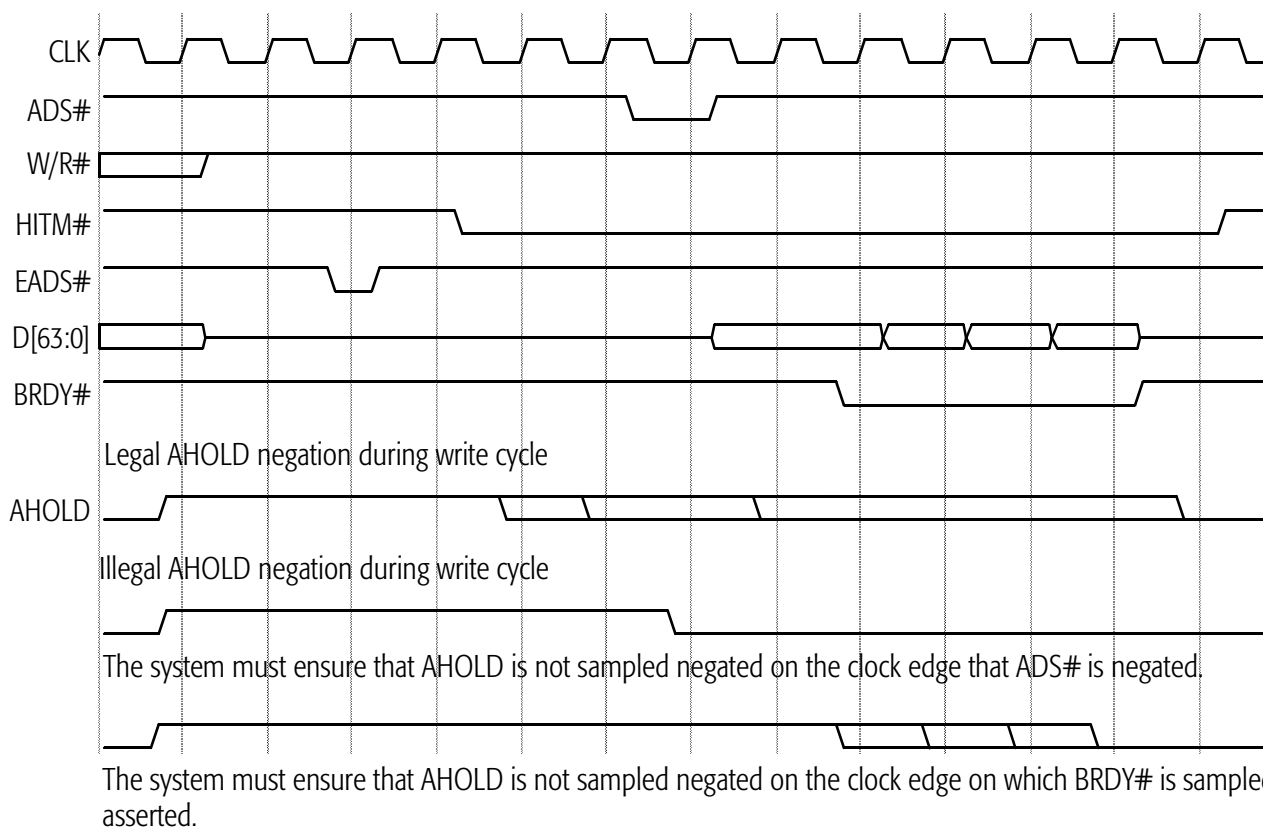
Figure 57. AHOLD Restriction
