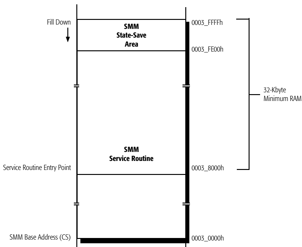
Figure 72. SMM Memory
