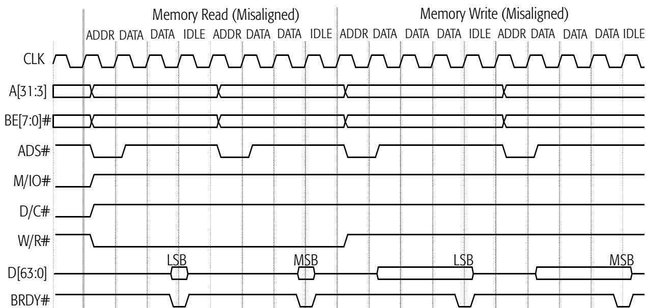
Figure 46. Misaligned Single-Transfer Memory Read and Write
