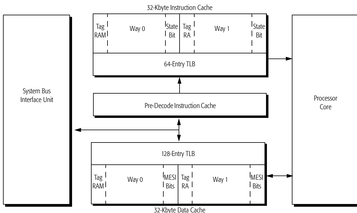
Figure 67. Cache Organization
