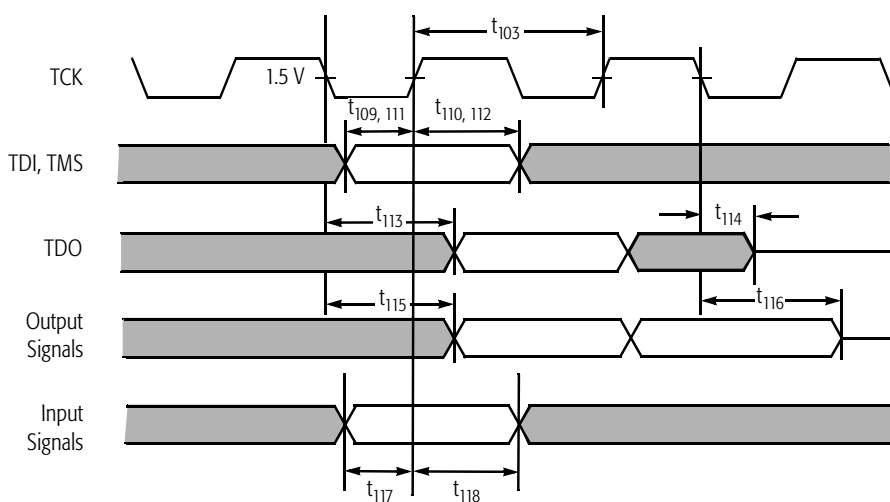
Figure 90. Test Signal Timing Diagram
