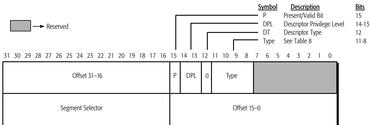
Figure 42. Gate Descriptor
