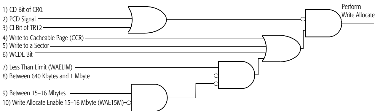
Figure 70. Write Allocate Logic Mechanisms and Conditions
