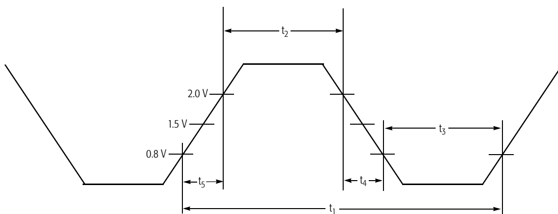
Figure 82. CLK Waveform
