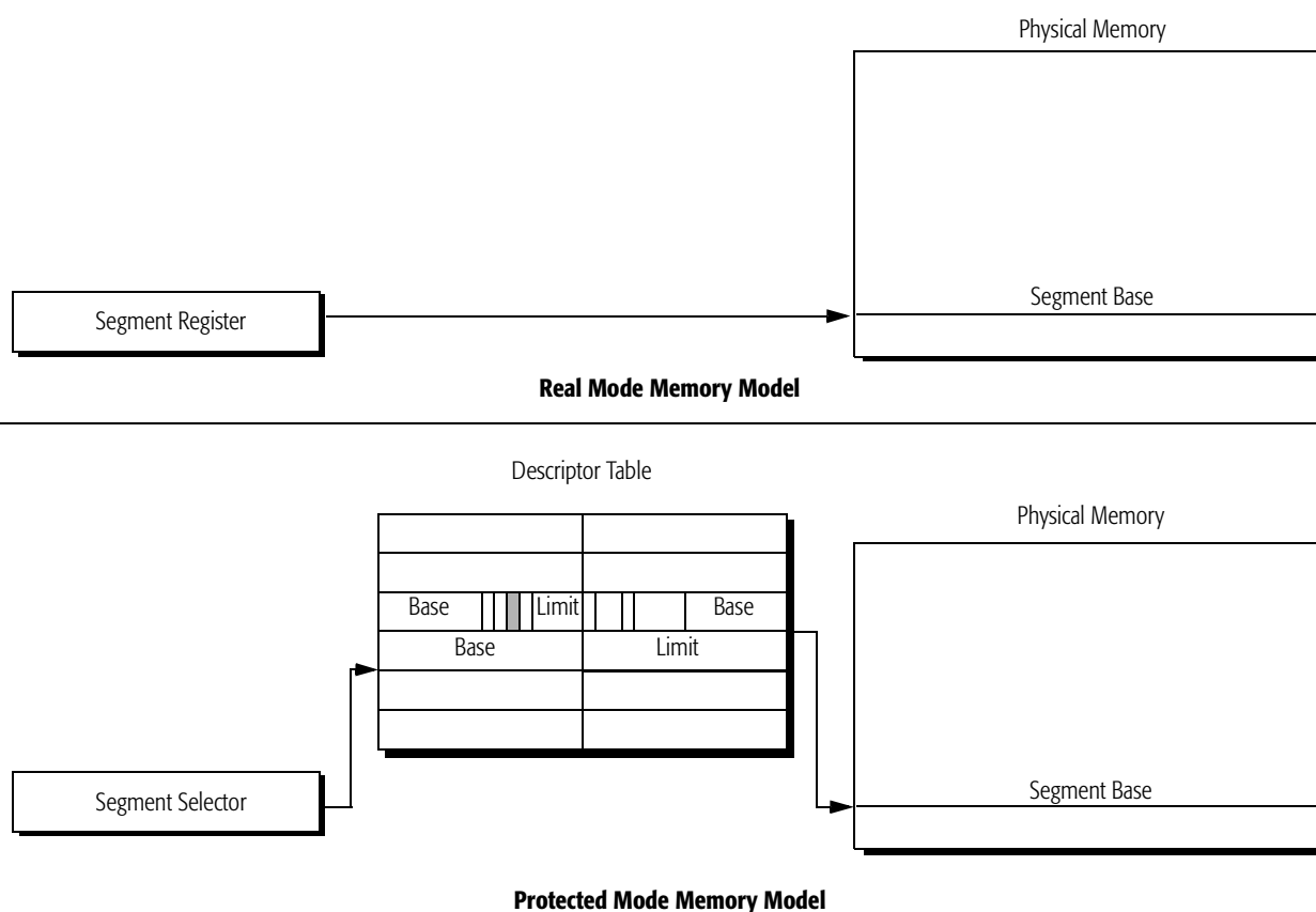
Figure 9. Segment Usage
