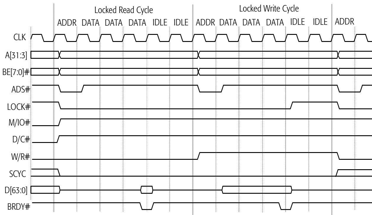
Figure 59. Basic Locked Operation
