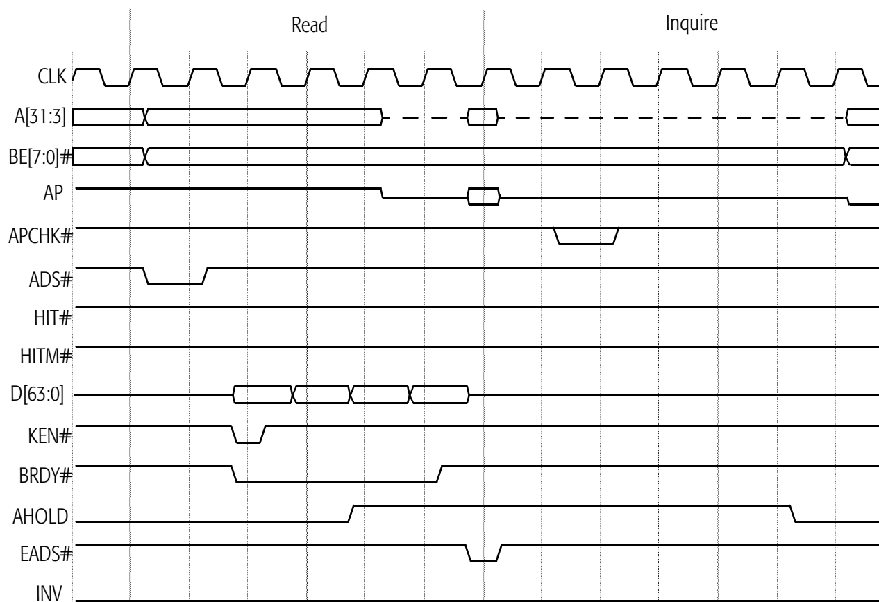
Figure 54. AHOLD-Initiated Inquire Miss
