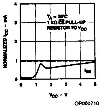
Typical Power-On Current Versus Power Supply
