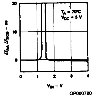
Access Time Change Versus Input Voltage
