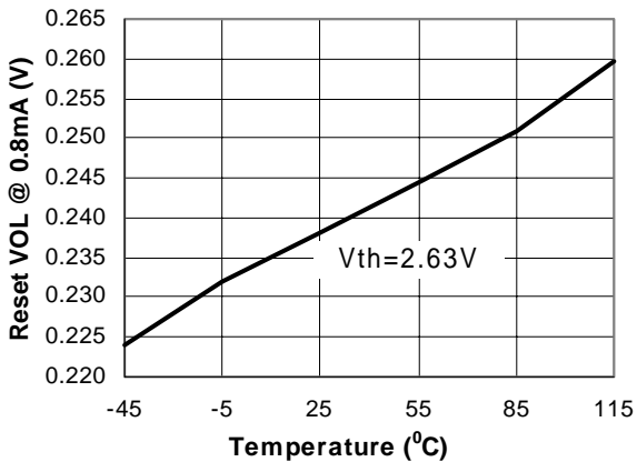
RESETB VOL vs Temperature
