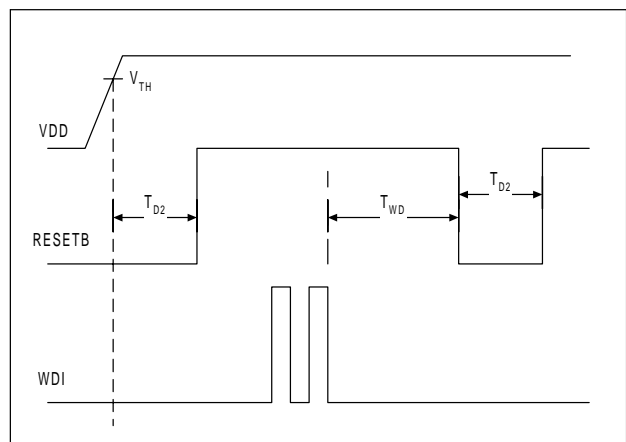
Watchdog Timing Diagram
