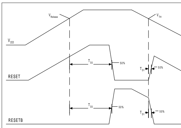
Reset Timing Diagram
