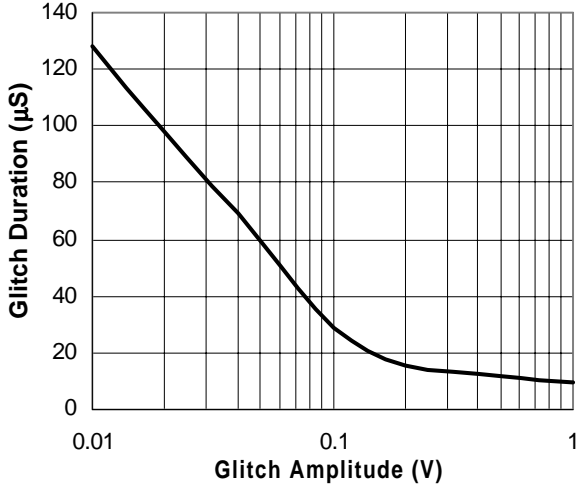
Glitch Rejection
