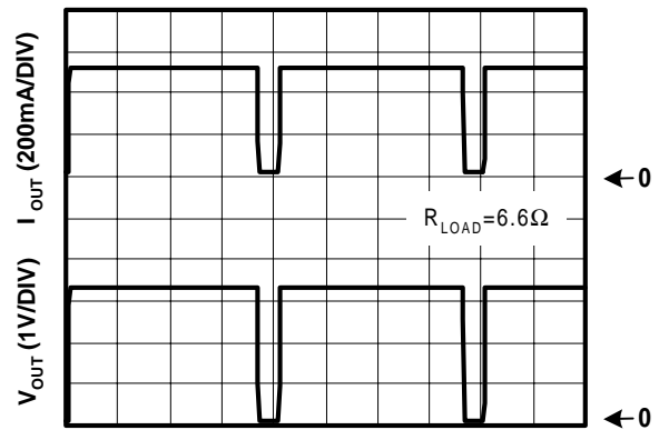
Overtemperature Shutdown
