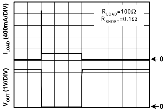
Short Circuit Response
