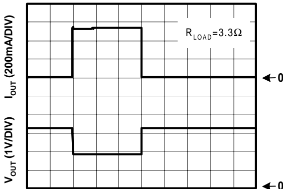
Current Limit Response
