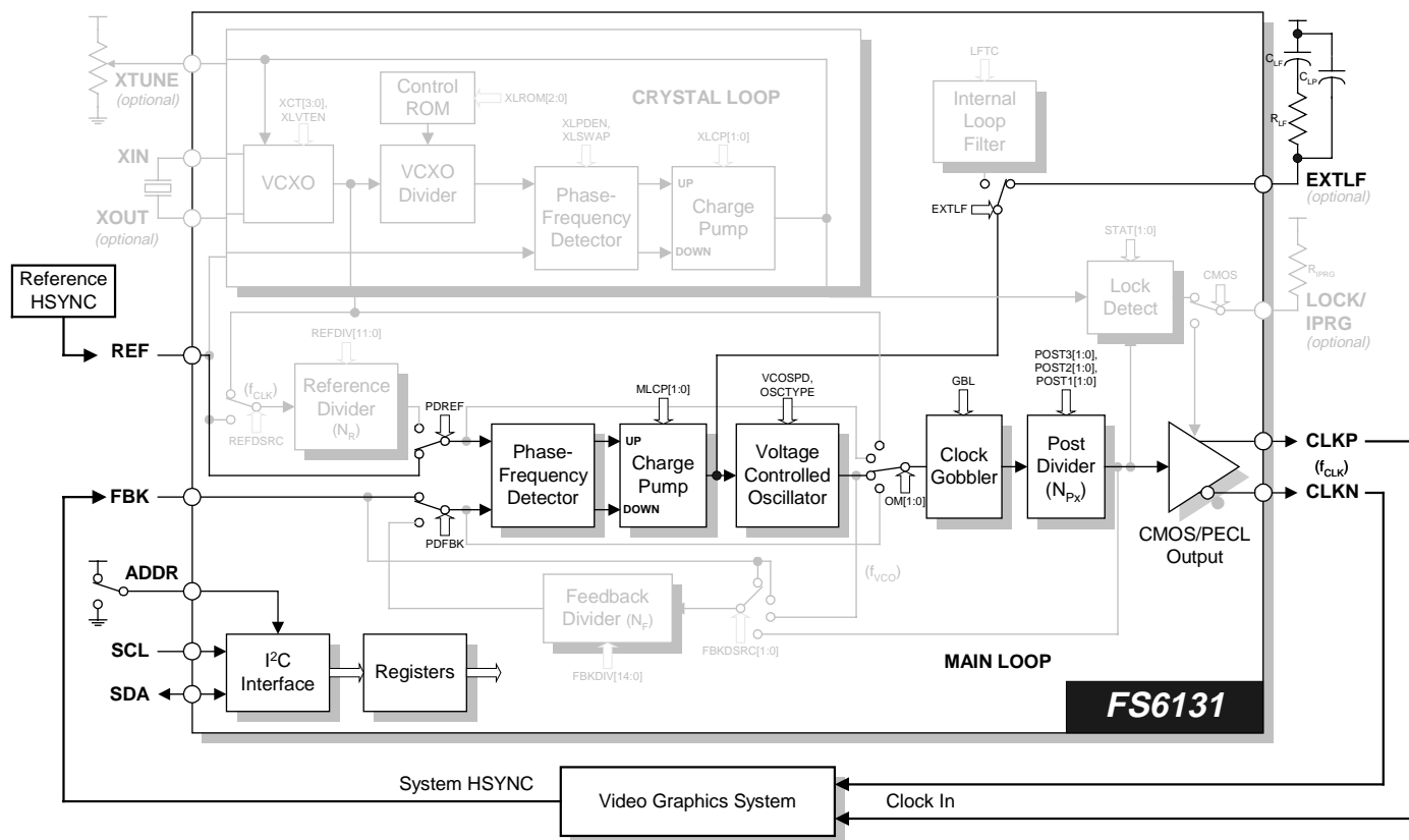
Figure 32: Block Diagram: Genlocking
