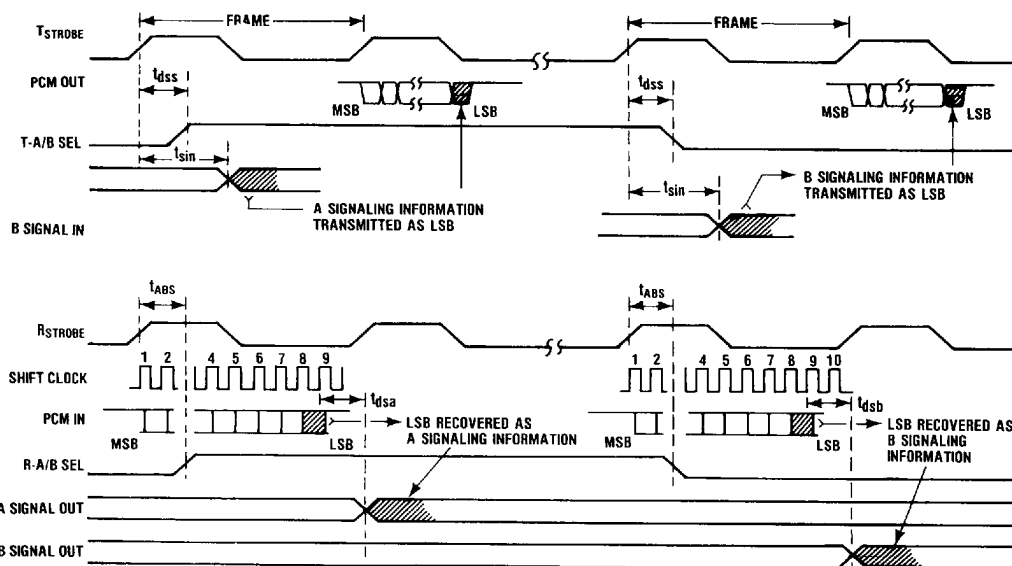
Figure 3A. Signaling Waveform Details
