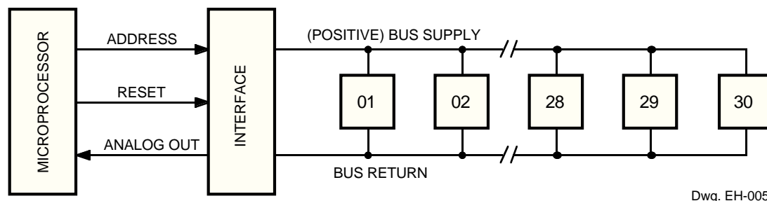
FIGURE 3 BUS INTERCONNECTION
