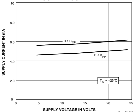
SUPPLY CURRENT
