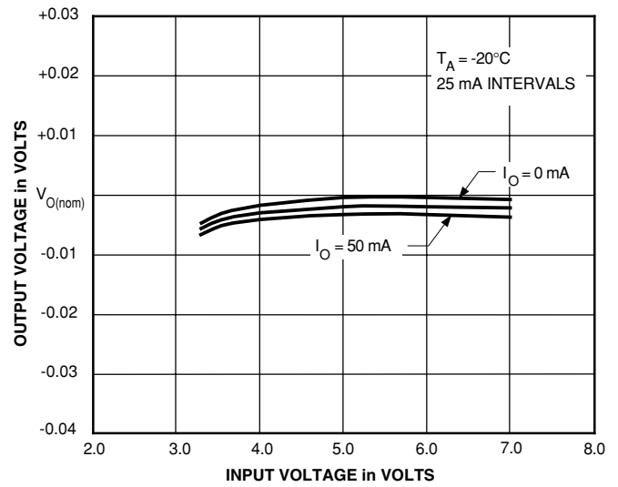
LINE REGULATION
