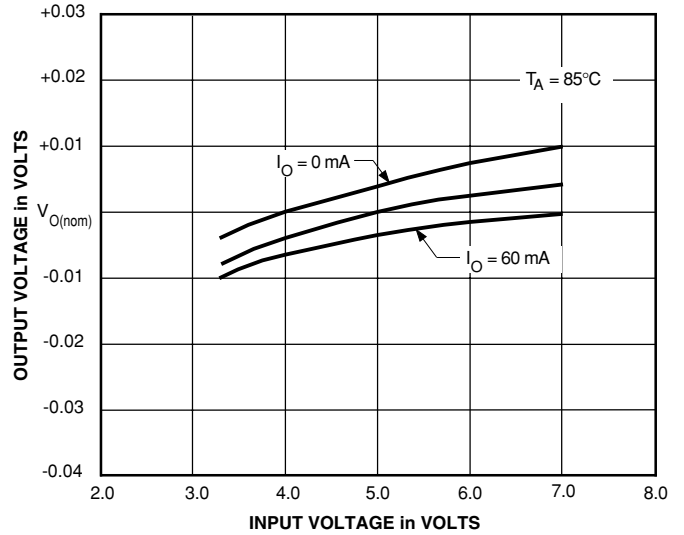
LINE REGULATION
