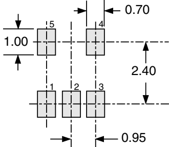
Dwg. MA-011-5 mm
