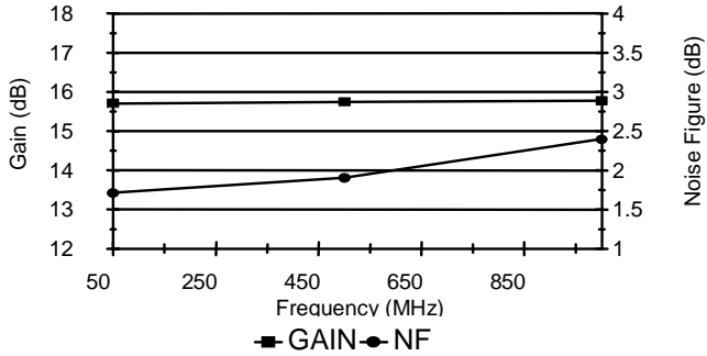
Gain and Noise Figure vs Frequency Tc = 25 deg C, V DD = +8V
