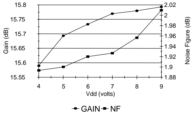
Gain and Noise Figure vs. Vdd Tc = 25 deg C, RF = 500 MHz
