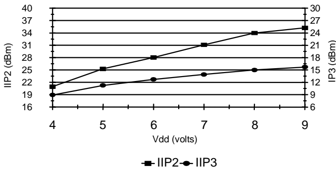
IIP2, IIP3 vs. Vdd Tc = 25 deg C
