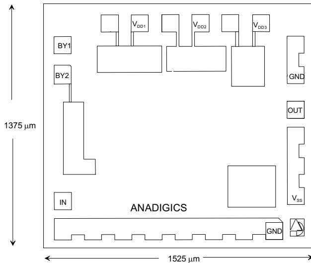
ATA30013 BOND PAD LAYOUT
